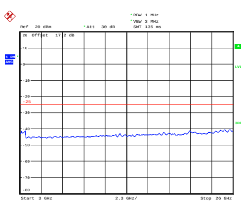
LTE Band 7 5MHz CH-Middle 3GHz~26GHz
