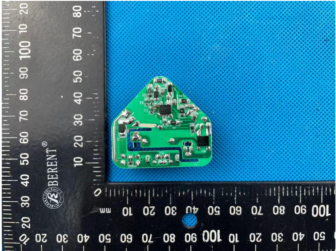
Charging cradle
