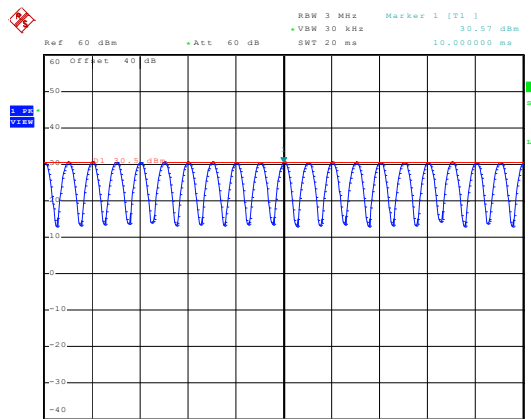
1880MHz - 80% AM
