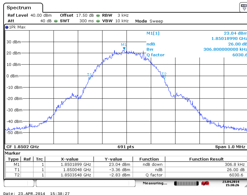
26dB Bandwidth Plot on Channel 512 (1850.2 MHz)
