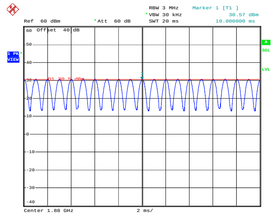
1880MHz - 80% AM
