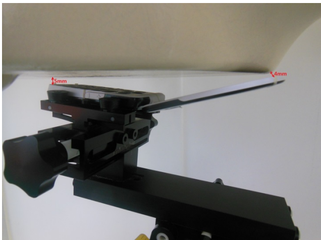
Left Cheek SAR in mouth area (Flip Open)
