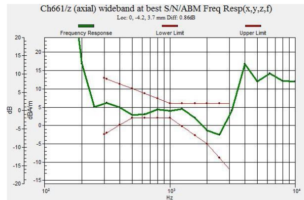
Fig 9.2 GSM1900 Ch661 for Sample #2
