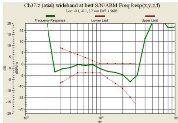
Fig 7.2 GSM900 Ch37
