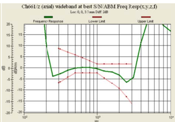
Fig 7.2 GSM1900 Ch661
