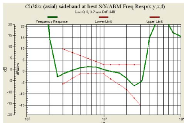
Fig 7.2 GSM900 Ch38
