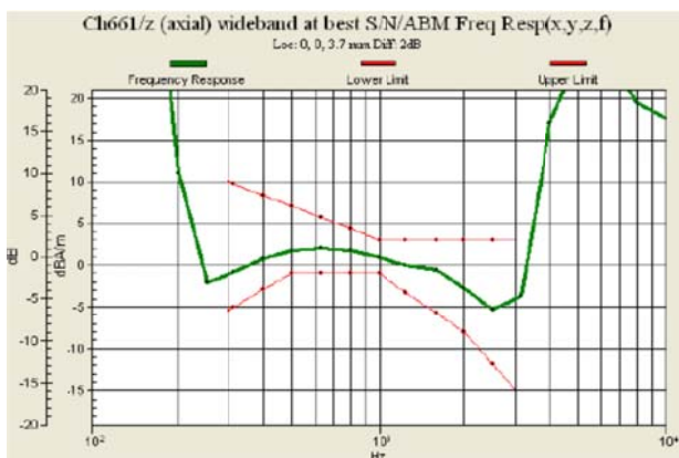
Fig 7.4 GSM1900 Ch661
