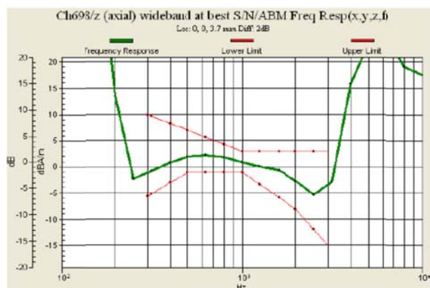
Fig 7.3 GSM1800 Ch698
