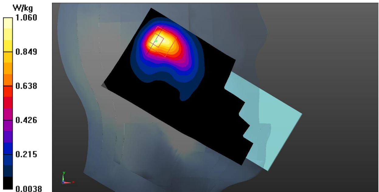
Fig.12 Wi-Fi 2.4G Head
