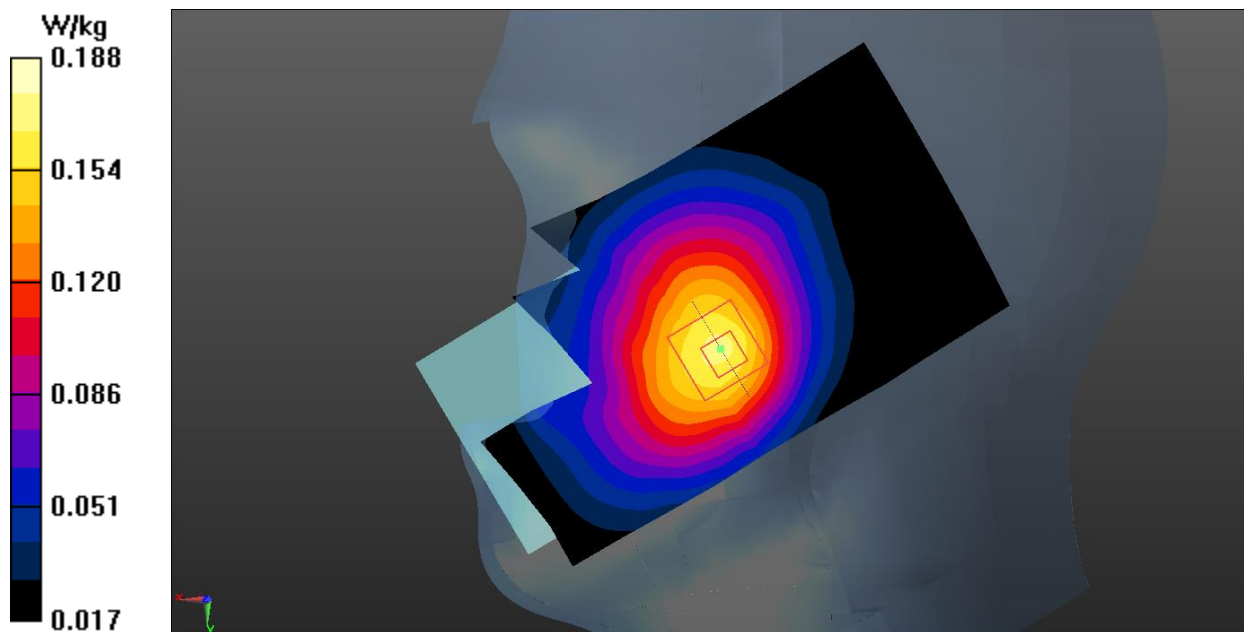
Fig.5 WCDMA850 Head
