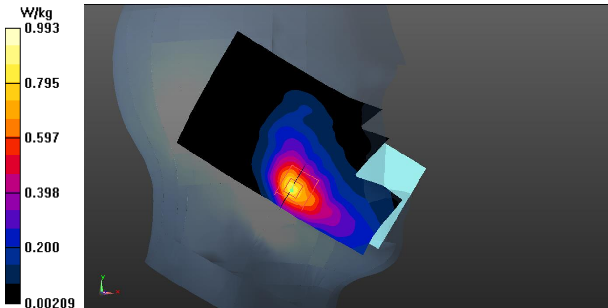
Fig.9 LTE Band 7 Head
