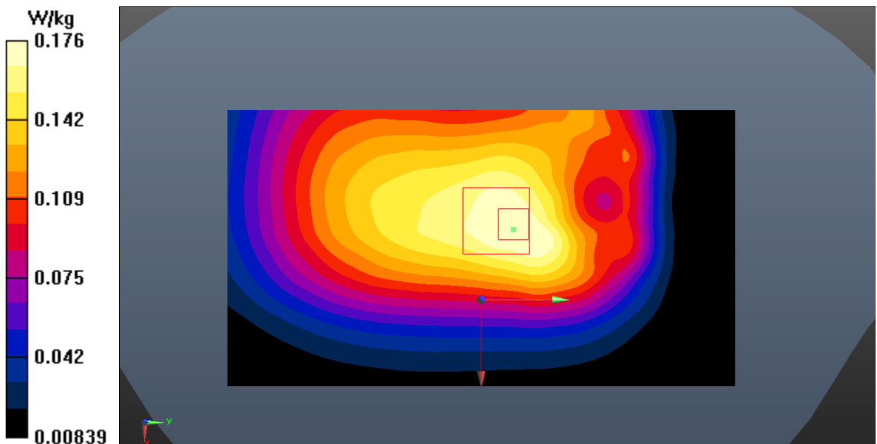
Fig.2 GSM850 Body
