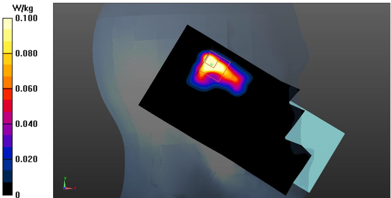
Fig.11 Bluetooth 2.4G Head
