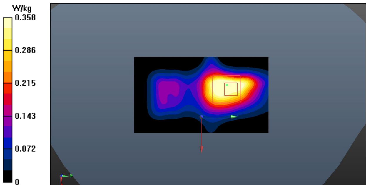
Fig.15 Wi-Fi 5G Body
