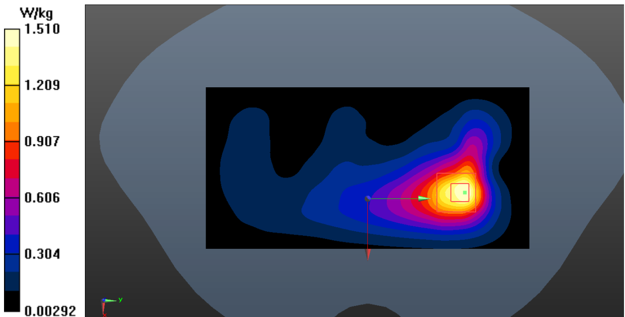
Fig.10 LTE Band 7 Body
