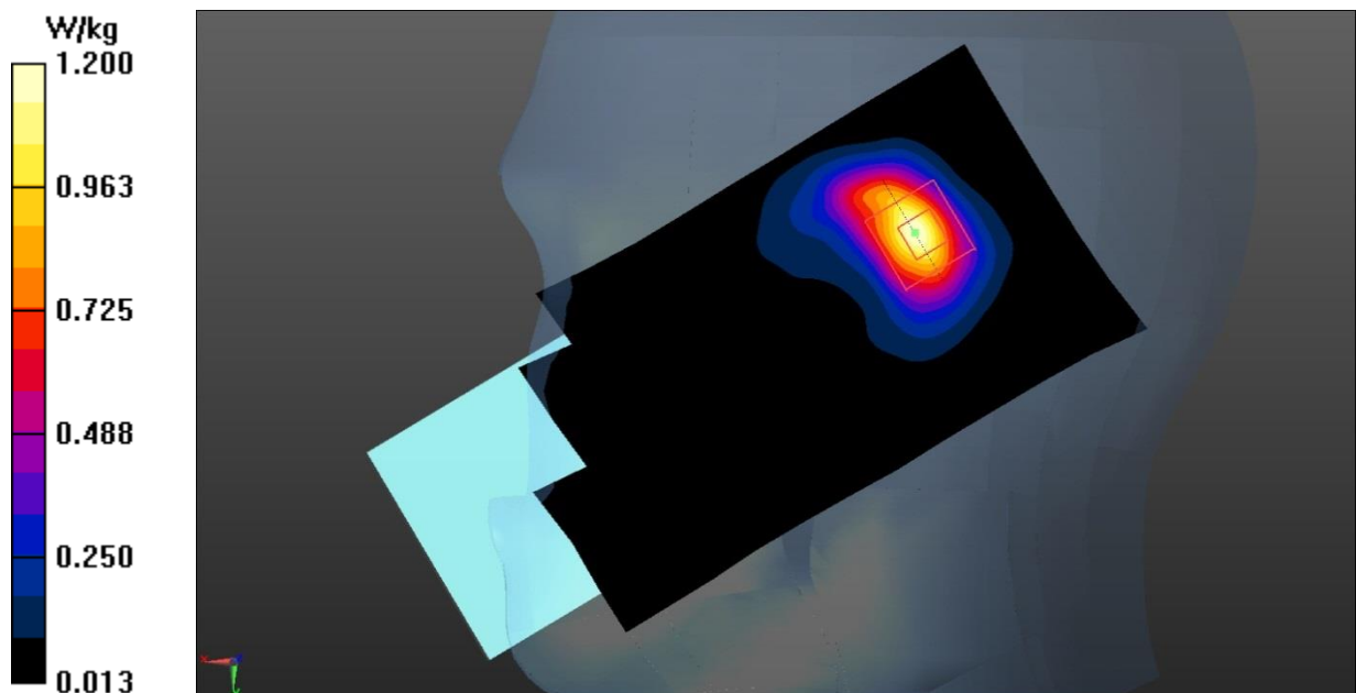
Fig.14 Wi-Fi 5G Head
