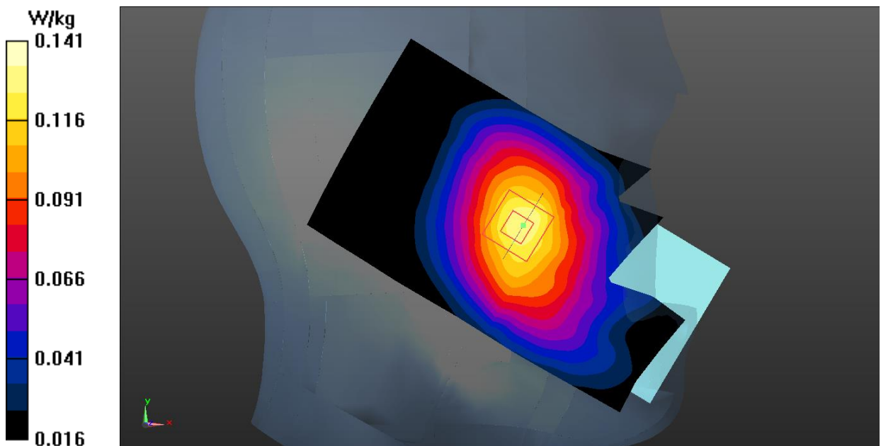
Fig.1 GSM850 Head
