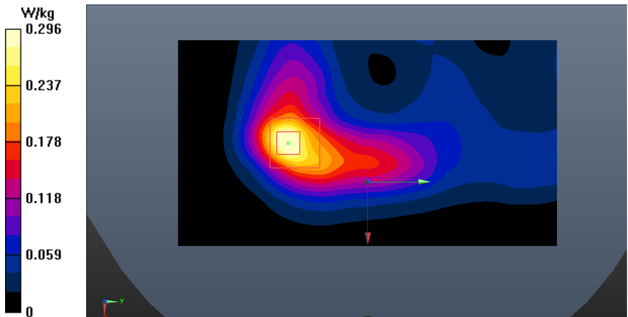
Fig.13 Wi-Fi 2.4G Body
