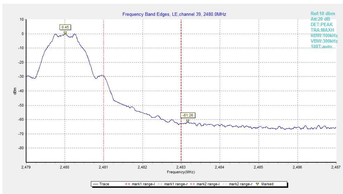
Fig.8 Band Edges (Ch 39), 1M
