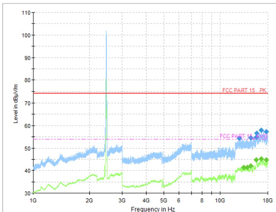
Fig.36 Radiated Spurious Emission (802.11b, CH11, 1GHz-18GHz)
