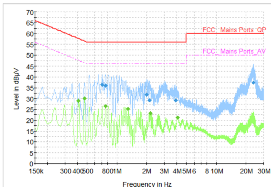
Fig.58 AC Power line Conducted Emission (Traffic, AE3, 240V)
