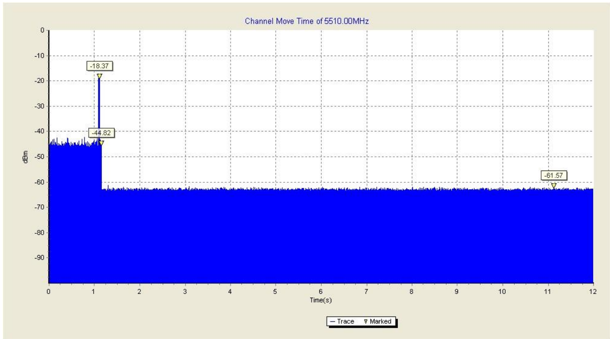
Fig.3 channel move time (HT40 Frequency Band: 5470MHz ~ 5725MHz)
