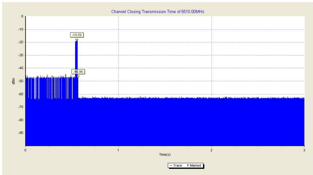
Fig.4 channel closing transmission time (HT40 Frequency Band: 5470MHz ~ 5725MHz)
