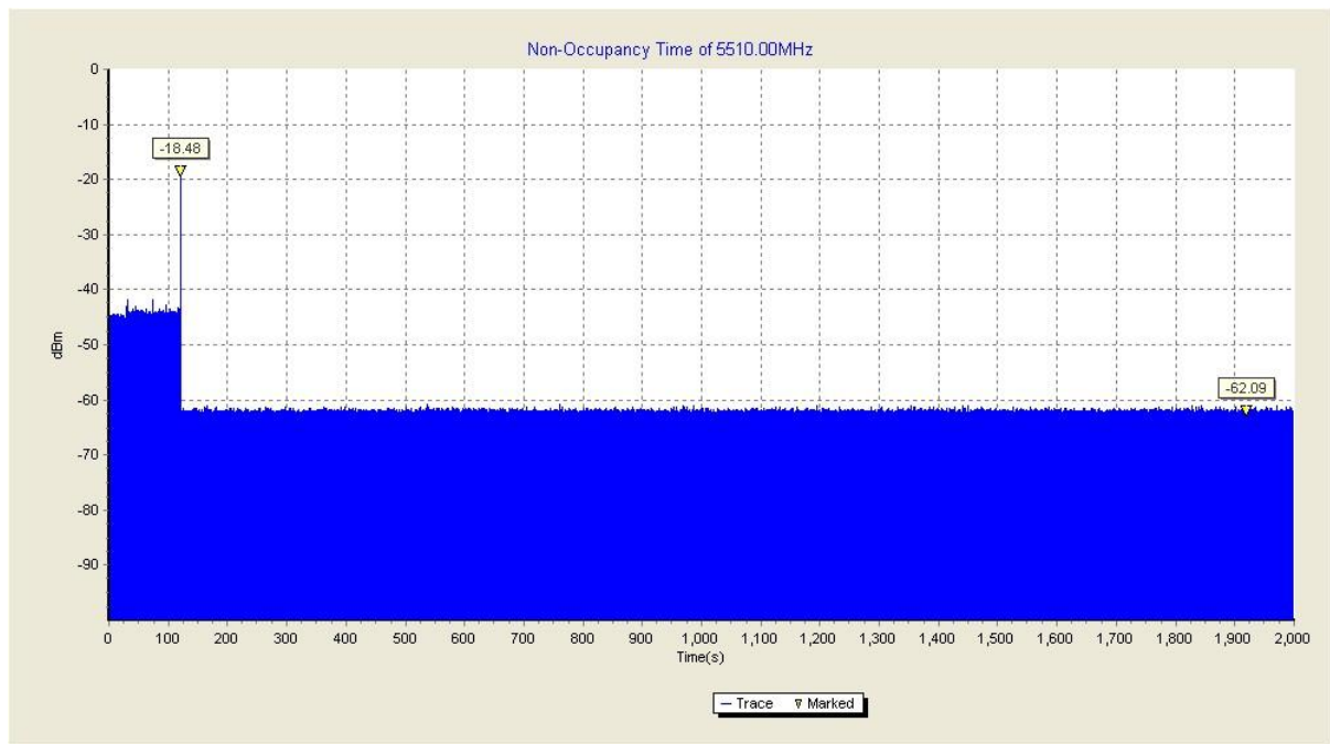
Fig.6 Non-Occupancy Period (HT40 Frequency Band: 5470MHz ~ 5725MHz)
