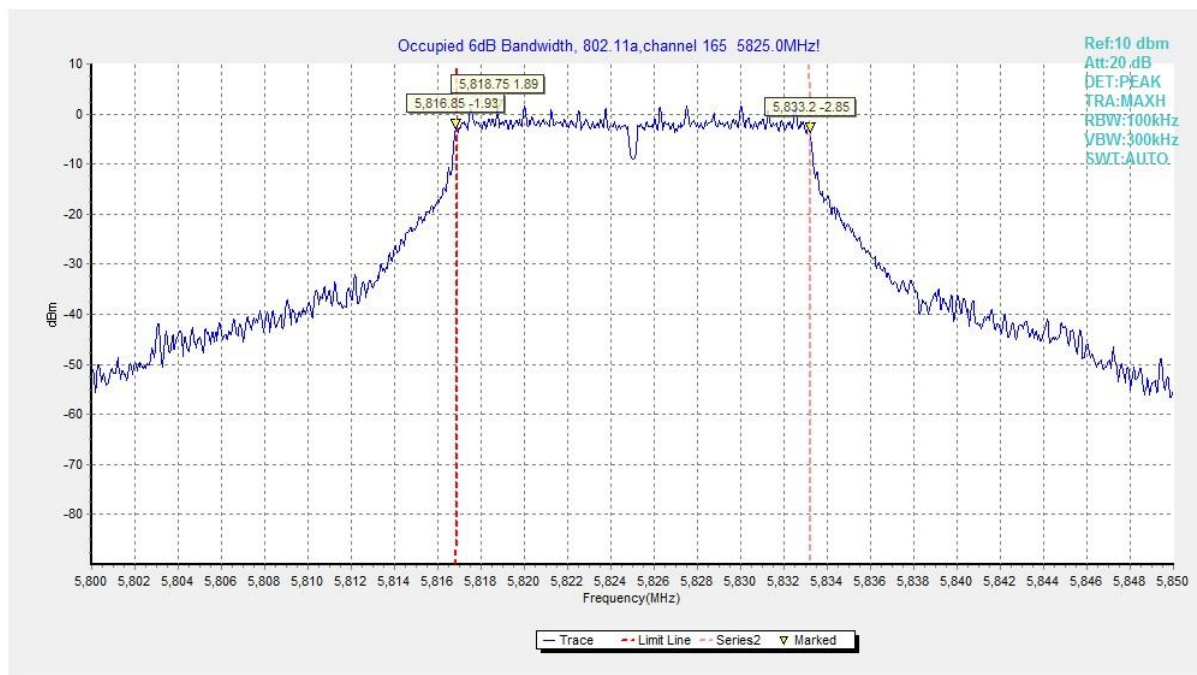
Fig. 19 Occupied 6dB Bandwidth (802.11a, 5825MHz)
