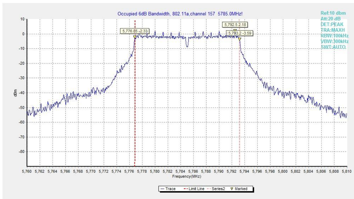
Fig. 18 Occupied 6dB Bandwidth (802.11a, 5785MHz)
