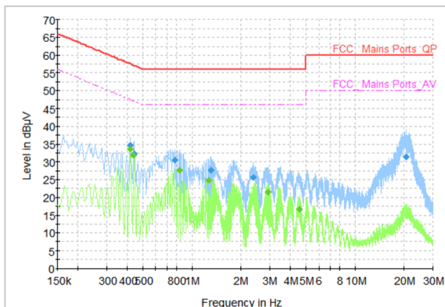
Fig. 80 AC Power line Conducted Emission (Idle, AE2, 240V)
