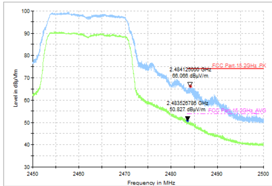
Fig.66 Radiated Restricted Band (802.11n-HT20, CH11, 2.45GHz~2.5GHz)
