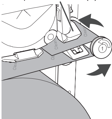
Paper end sensor (2)
