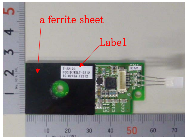
External Photos (For limited use, there is no metal shield.)
