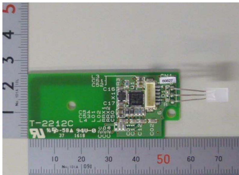
Internal Photos (For limited use, there is no metal shield.)
