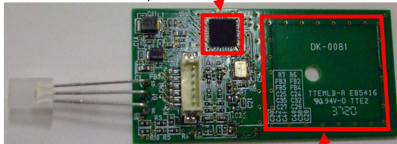
RFID RW Board DK-0081 Top
