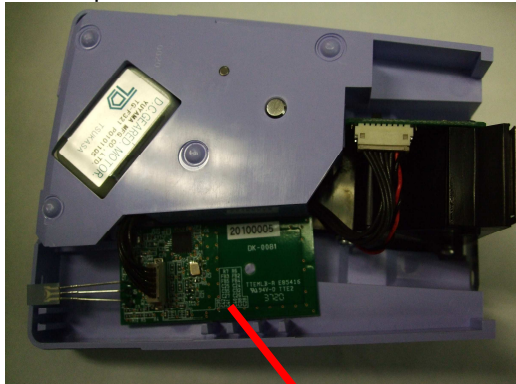
RFID RW Board DK-0081 Top
