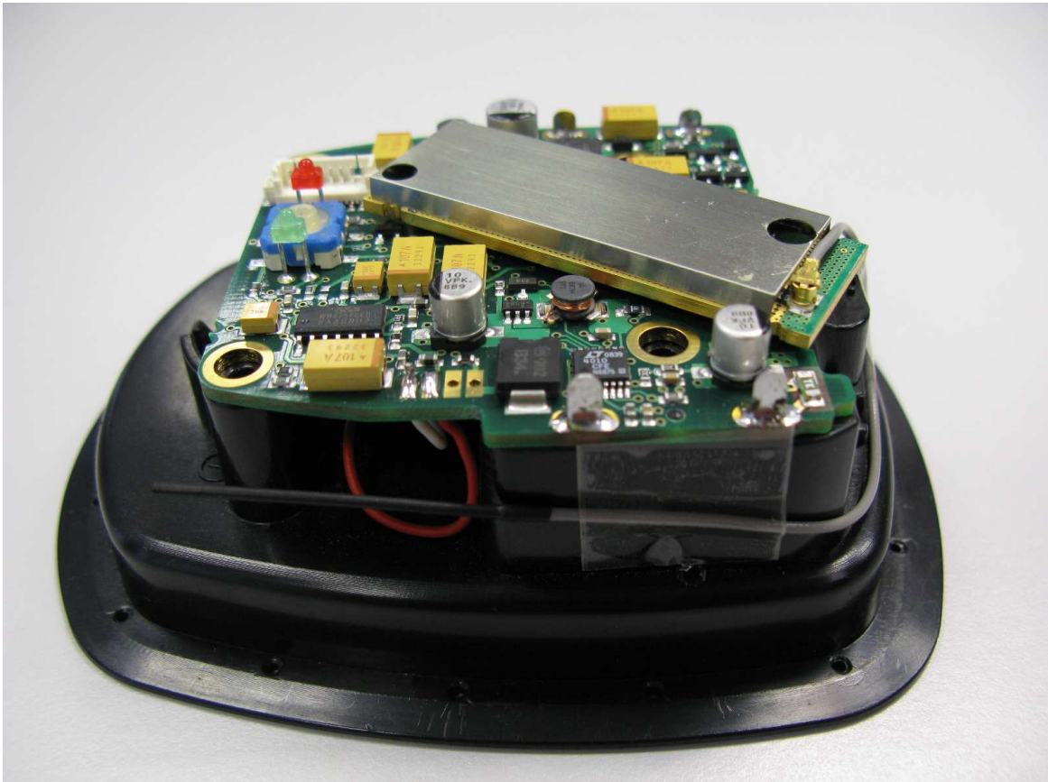
Figure 4: Integration in headphone module with external antenna
