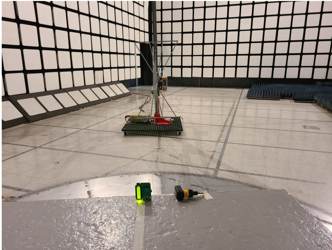
Radiated Emissions at 3 m Distance (30-1000 MHz) Orthogonal Position 2
