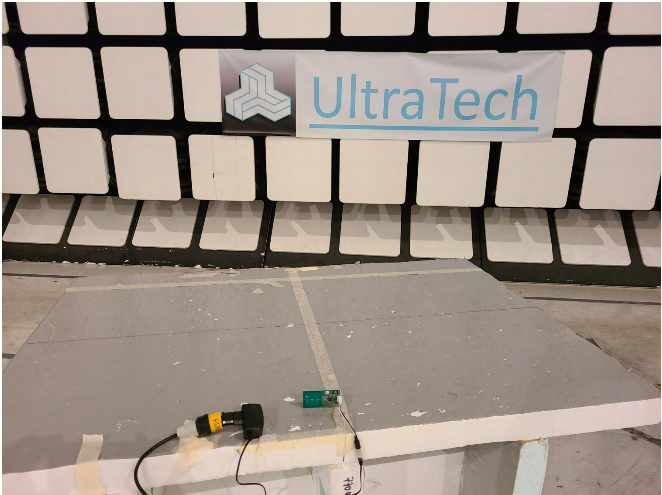
Radiated Emissions at 3 m Distance (30-1000 MHz) Orthogonal Position 3
