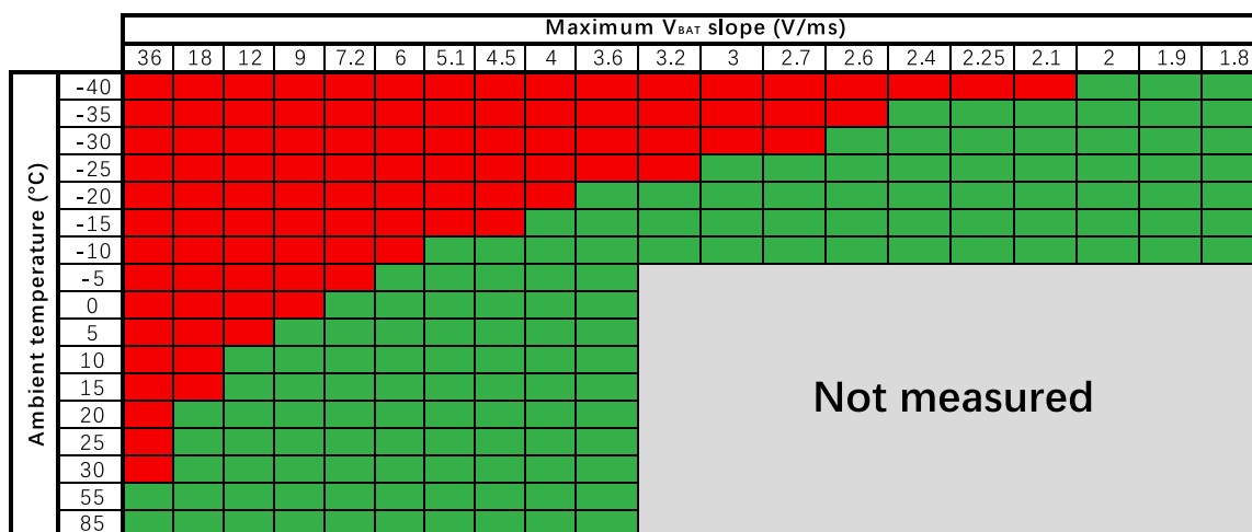
Fig 13. Maximum V_{BAT} slope vs temperature
