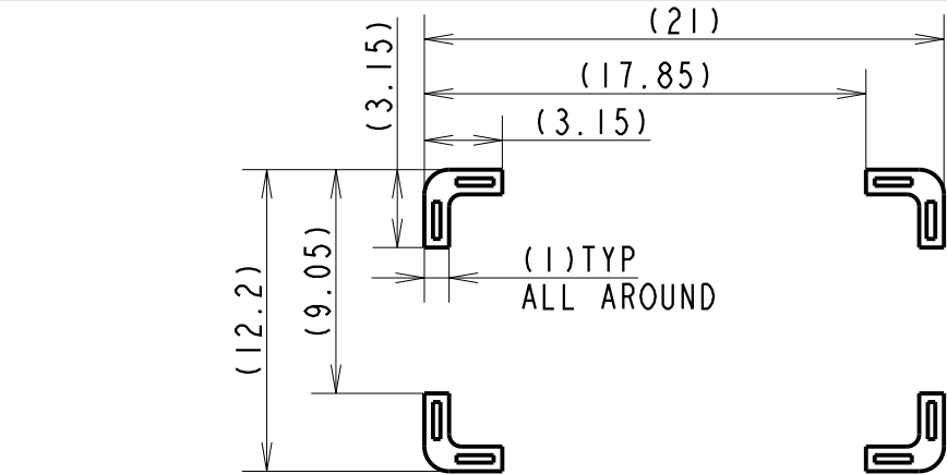
SOLDER PAD LAYOUT
