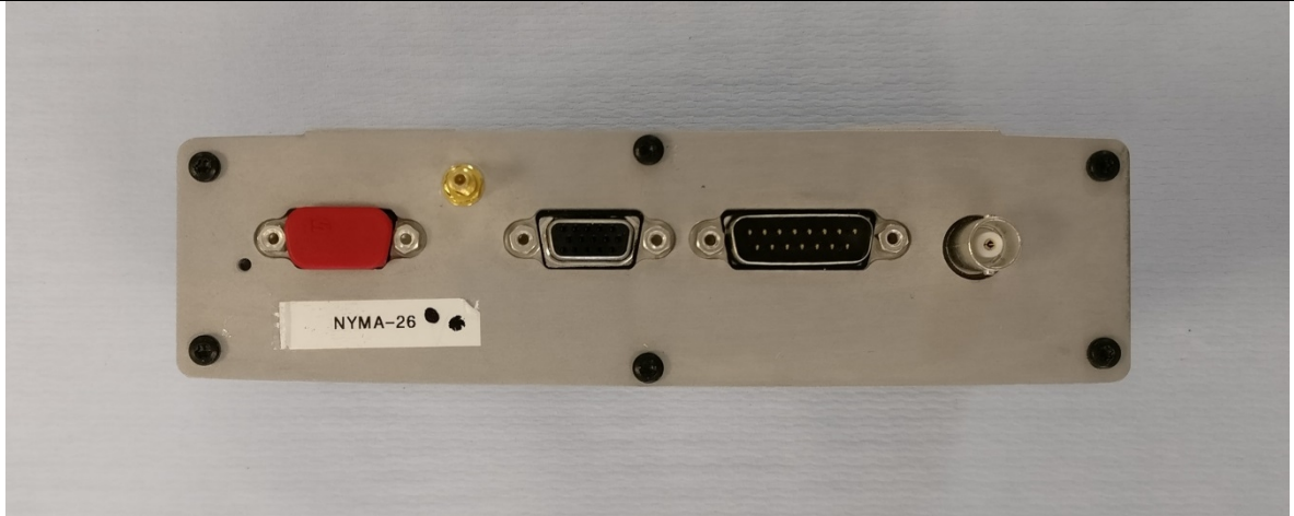
MDT-500-2 Connector View
