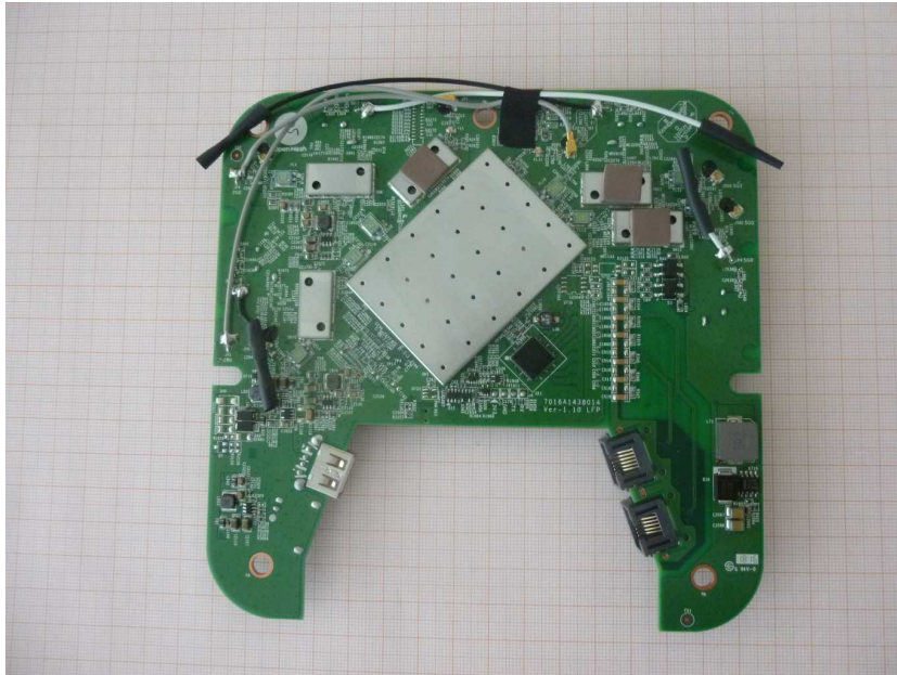
Photo 3 EUT board rear view
