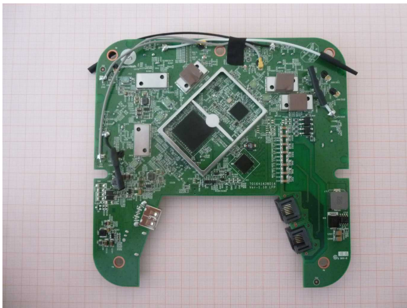
Photo 4 EUT board rear view without shielding
