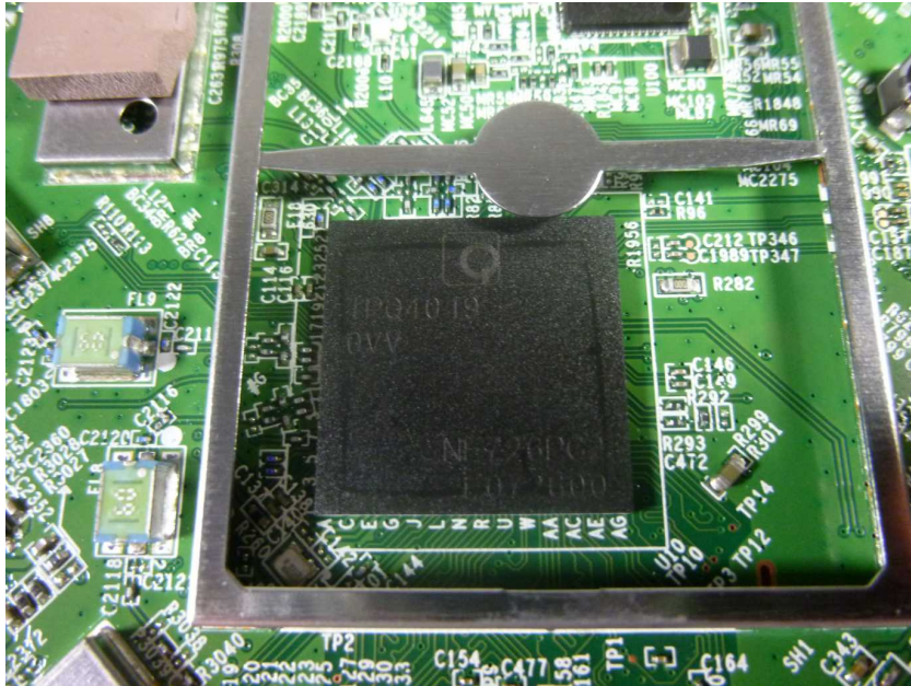
Photo 7 EUT IC detailed view
