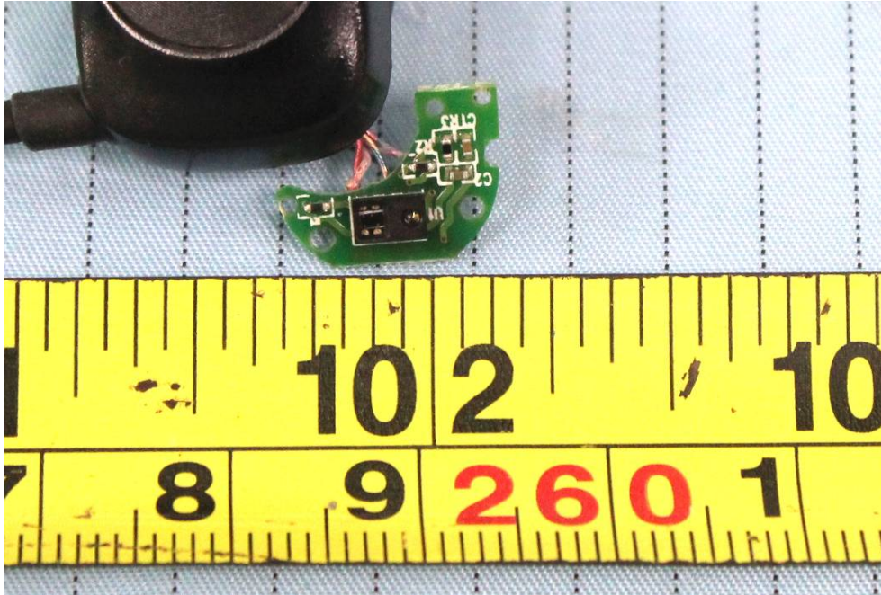
EUT – Ear Board Top View
