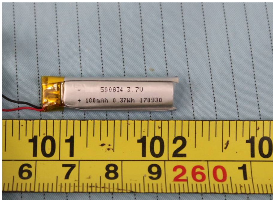
EUT –Battery Front View
