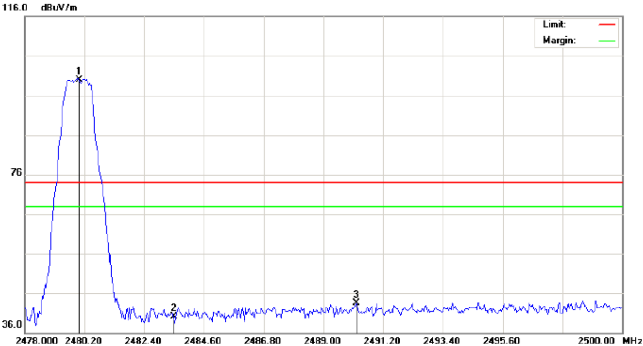
TEST PLOT OF BAND EDGE FOR HIGH CHANNEL (1Mbps)-Horizontal
