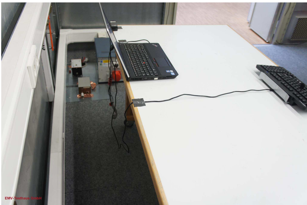
Picture 6: EUT test setup conducted emission test (rear view)
