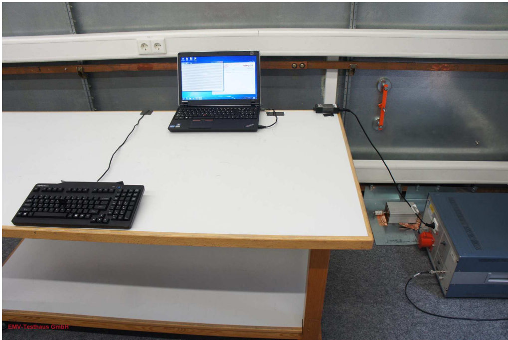
Picture 5: EUT test setup conducted emission test (front view)
