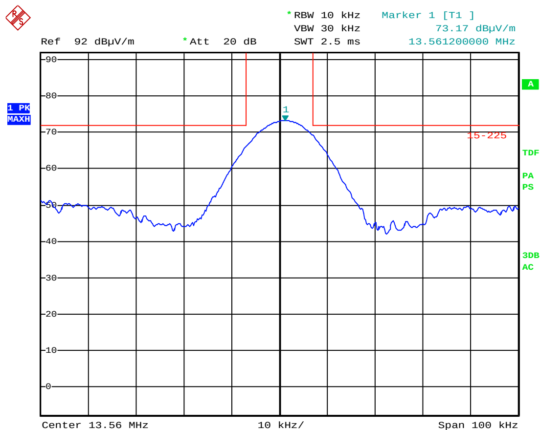
Picture 25: Spectrum mask for 13.56 MHz @ 3m distance (10 kHz BW), antenna 2
