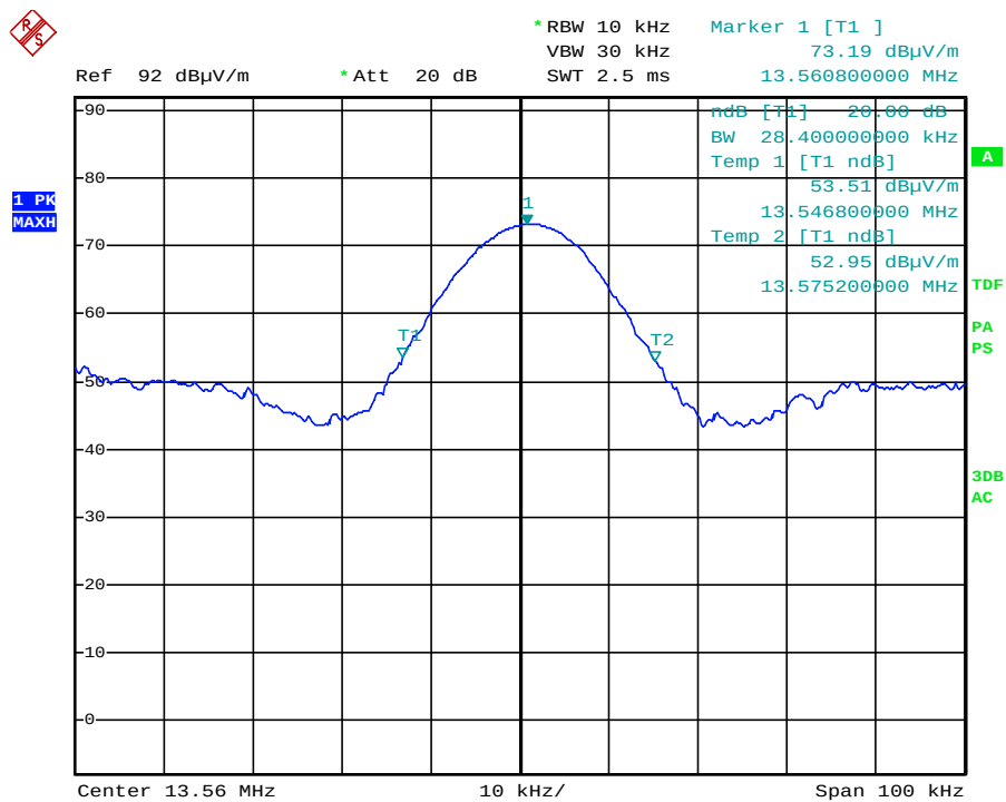
Picture 30: -20 dB emission bandwidths, antenna 2
