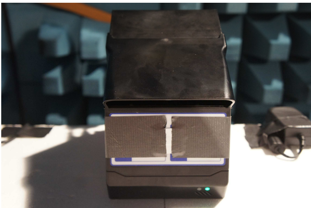
Picture 12: EUT antenna 2, position 3
