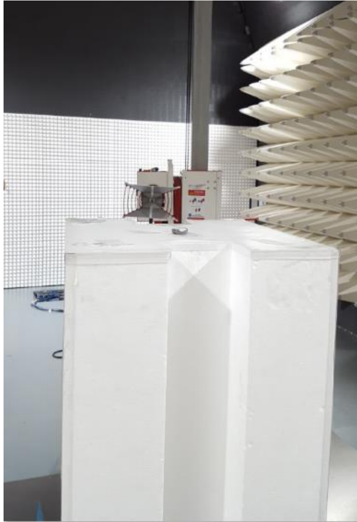
Figure B5. Radiated Setup 2
