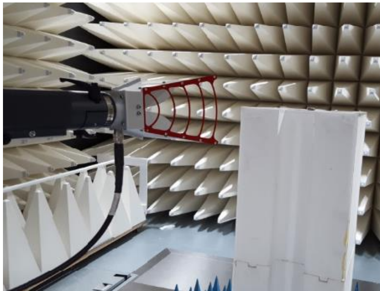
Figure B4. Radiated Setup 1
