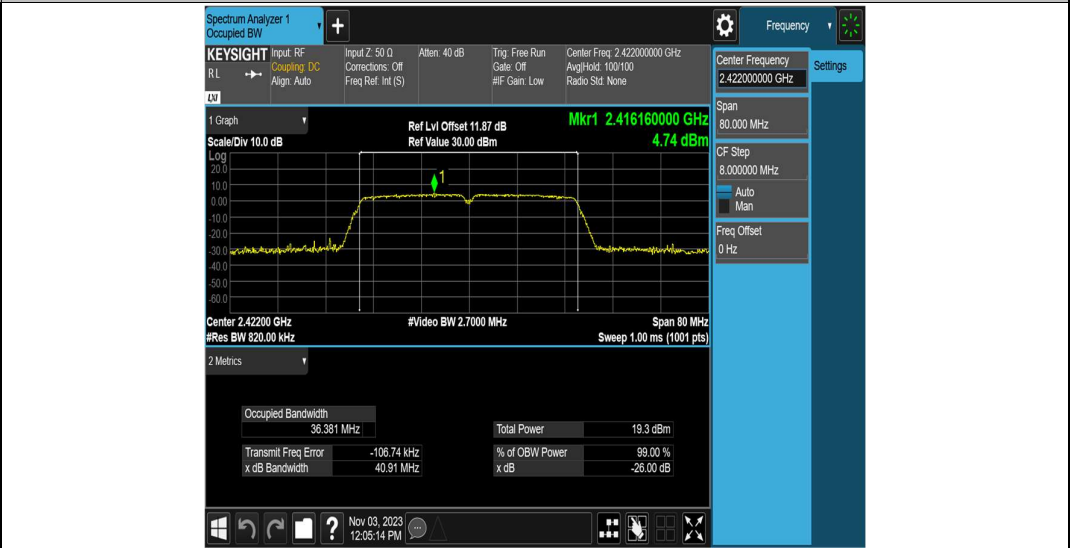
11N40SISO_Ant1_2422
