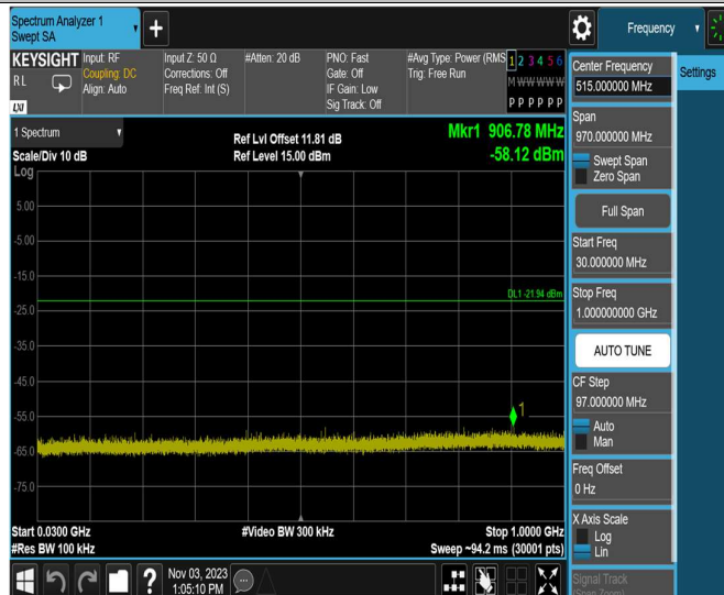
11N40SISO_Ant1_2452_30~1000
