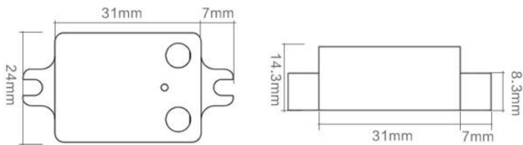
Outline Drawing
