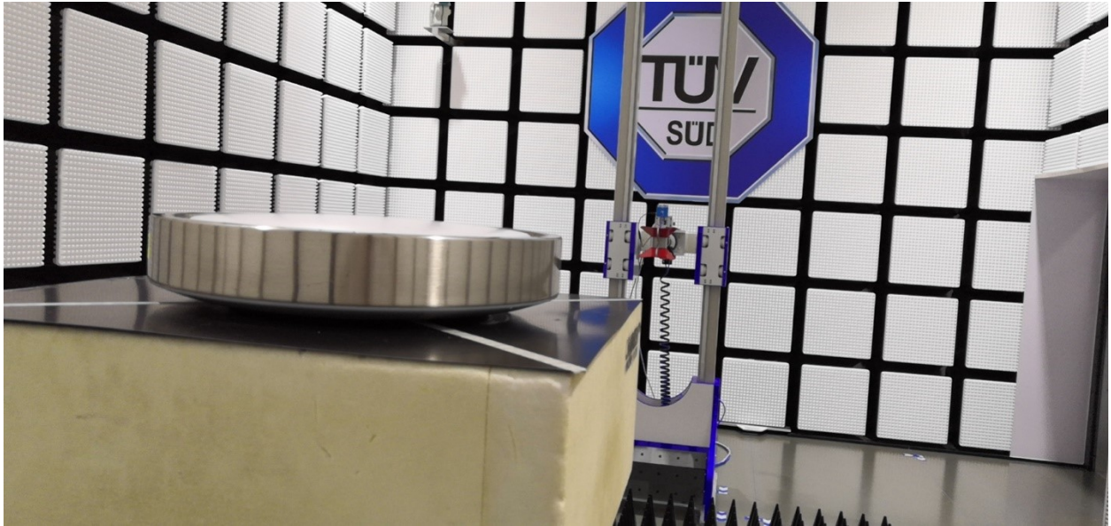
Radiated Emission test (2# Test Site) 1-18GHz
