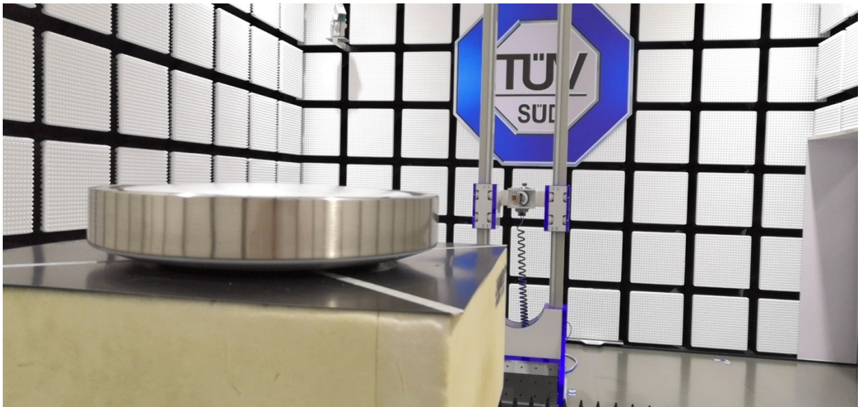
Radiated Emission test (2# Test Site) 18-40GHz
