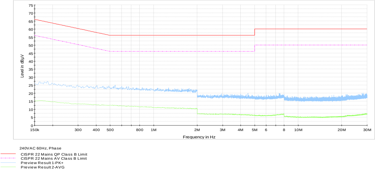
Plot 8.1-3: Conducted emissions on phase line
