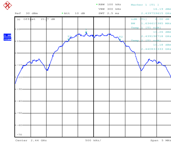
Figure 8.2-2: 6 dB bandwidth – Tx 2440 MHz
