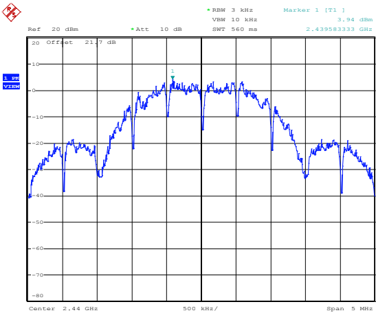
Figure 8.5-2: PSD plot – Tx 2440 MHz
