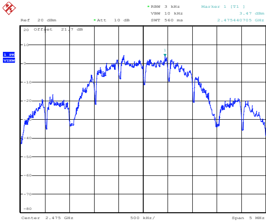
Figure 8.5-3: PSD plot – Tx 2475 MHz
