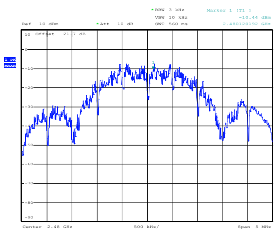
Figure 8.5-4: PSD plot – Tx 2480 MHz
