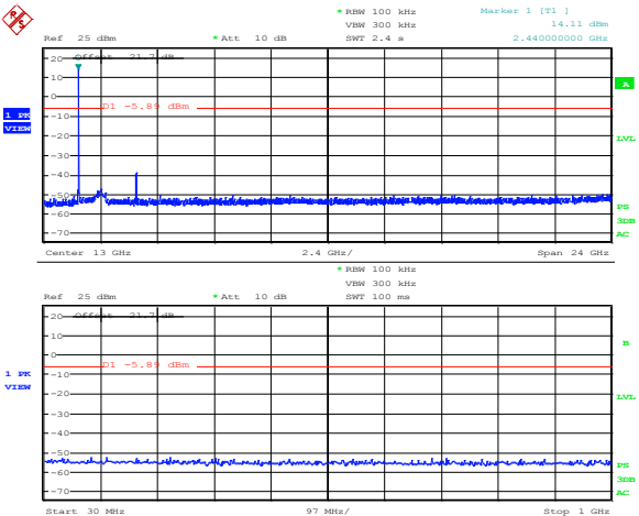
Figure 8.4-10: Conducted spurious, mid channel
