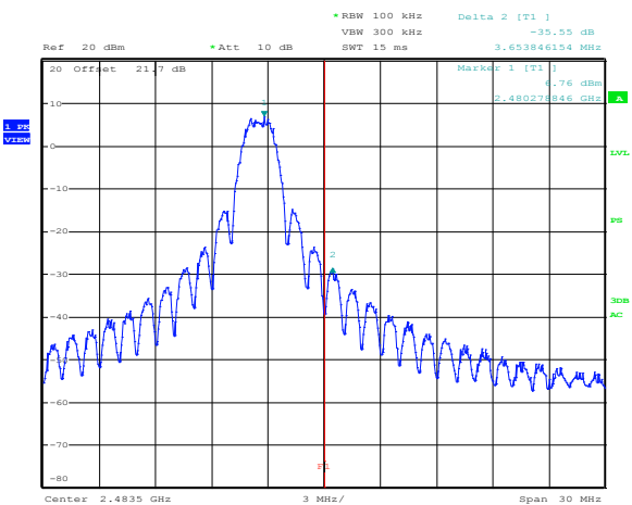
Figure 8.4-8: Conducted spurious emissions for High channel
