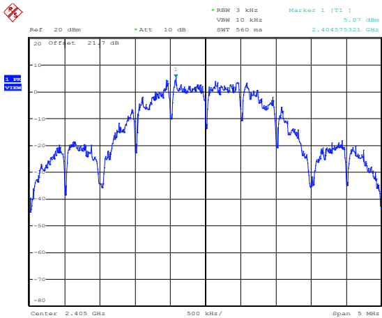
Figure 8.5-1: PSD plot – Tx 2405 MHz
