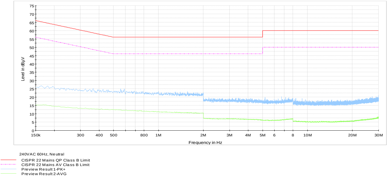
Plot 8.1-4: Conducted emissions on neutral line
