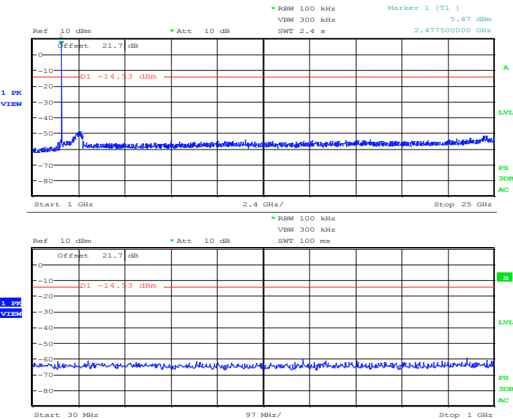
Figure 8.4-11: Conducted spurious emissions, High channel
