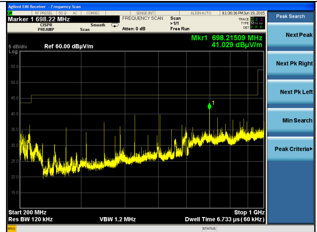
200-1000 MHz Horizontal
