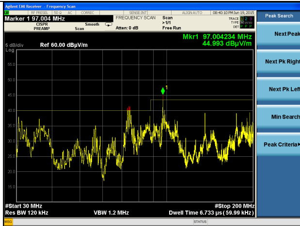
30-200 MHz Vertical
