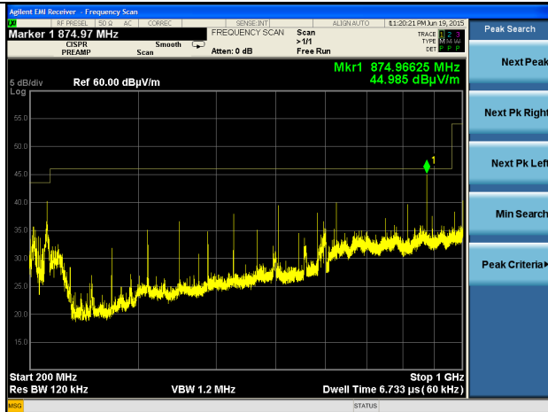
200-1000 MHz Vertical
