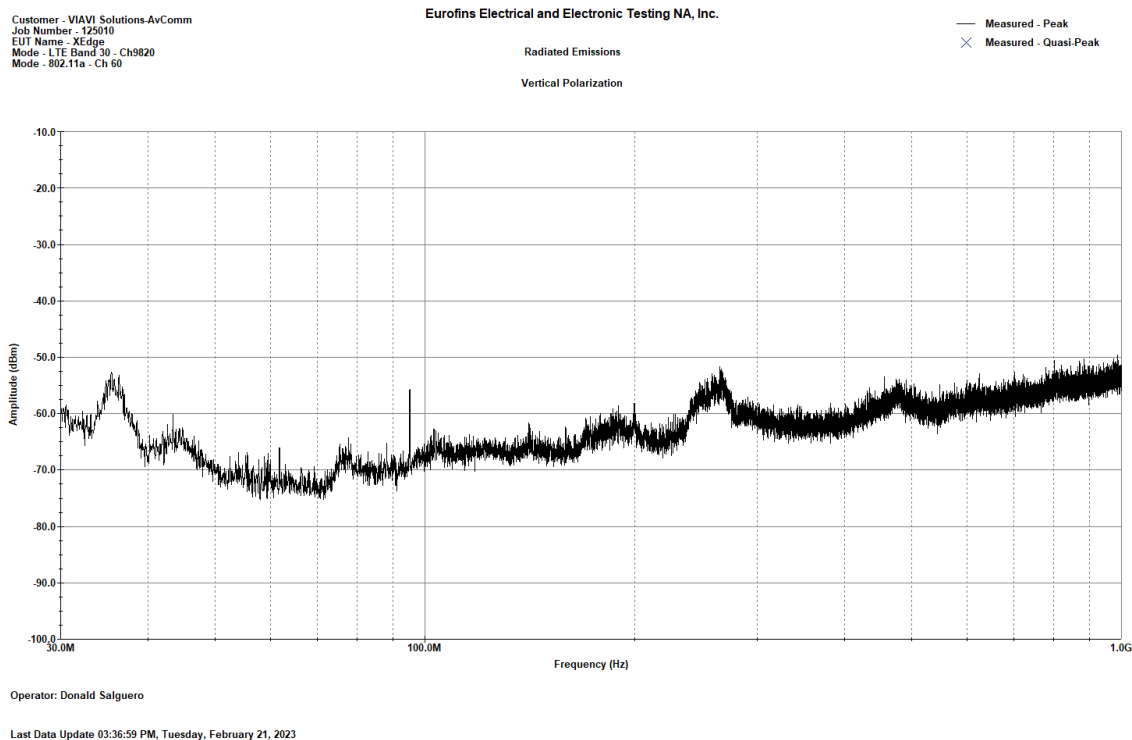
Figure 34. Colocation Radiated Emissions_LTE B30_WiFi ch60_30MHz-1GHz
