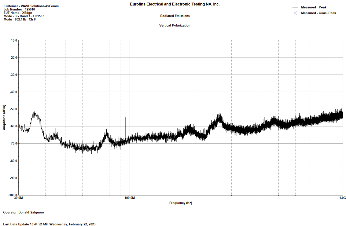
Figure 10. Colocation Radiated Emissions_3G B4_WiFi ch6_30MHz-1GHz
