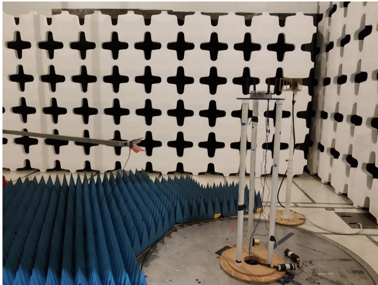
Figure 2. Radiated Emissions Test Setup, 1-18 GHz
