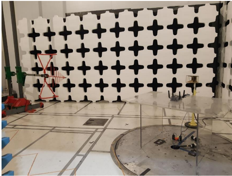
Figure 1. Radiated Emissions Test Setup, 30-1000 MHz
