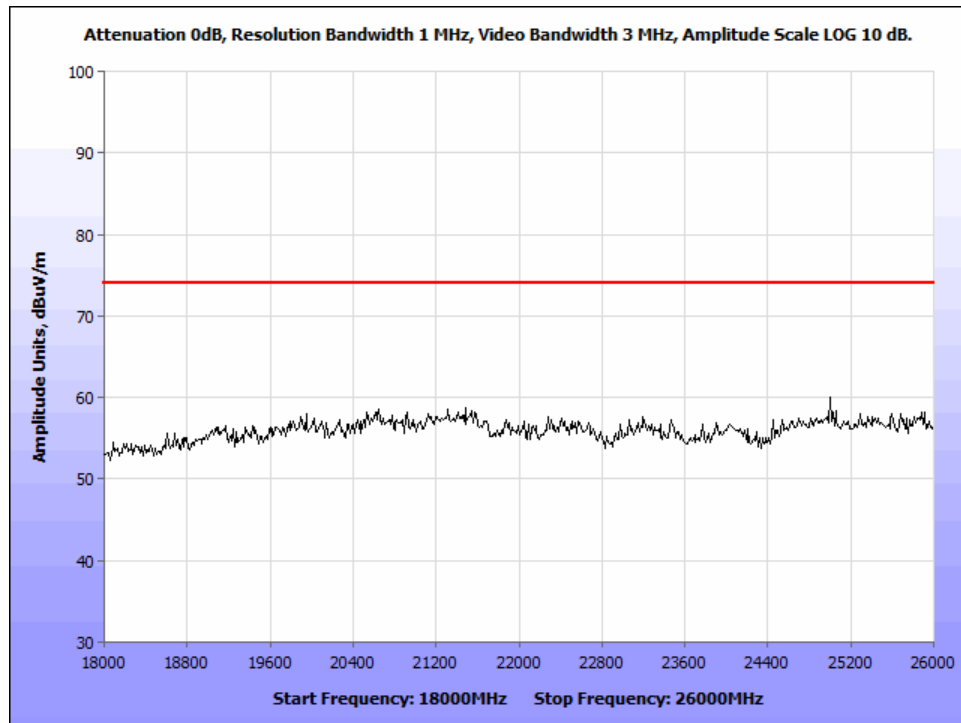
Figure 15: Radiated Emissions, Peak, 18 GHz – 26 GHz
