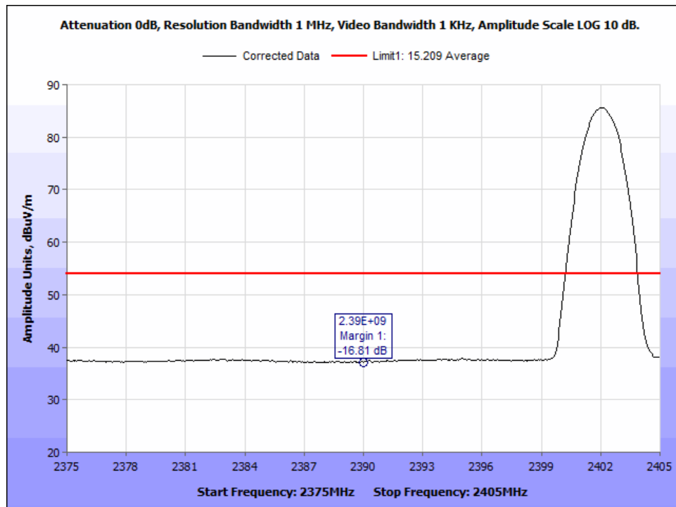
Figure 19: Average Radiated Bandedge @2390MHz – pi/4 DQPSK 2402MHz.
