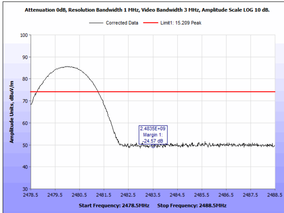
Figure 26: Peak Radiated Bandedge @2483.5MHz - 8DPSK 2480MHz.
