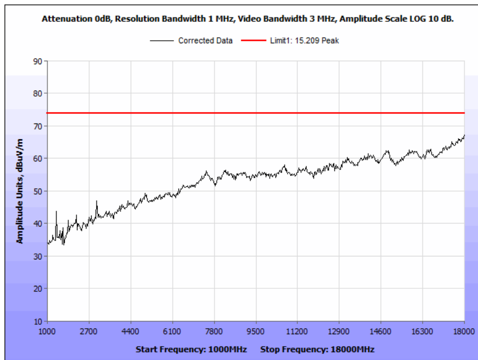
Figure 14: 15.209 Peak Radiated Emissions - GFSK 2480MHz - 1-18GHz.
