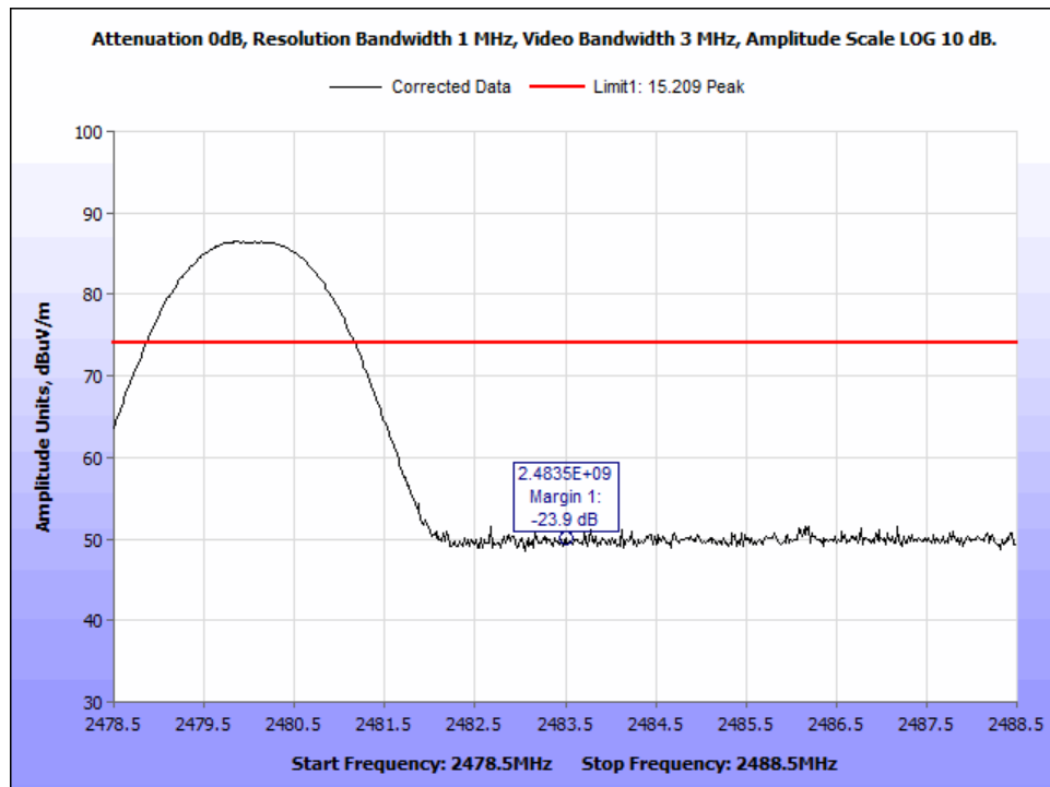
Figure 27: Peak Radiated Bandedge @2483.5MHz - GFSK 2480MHz.
