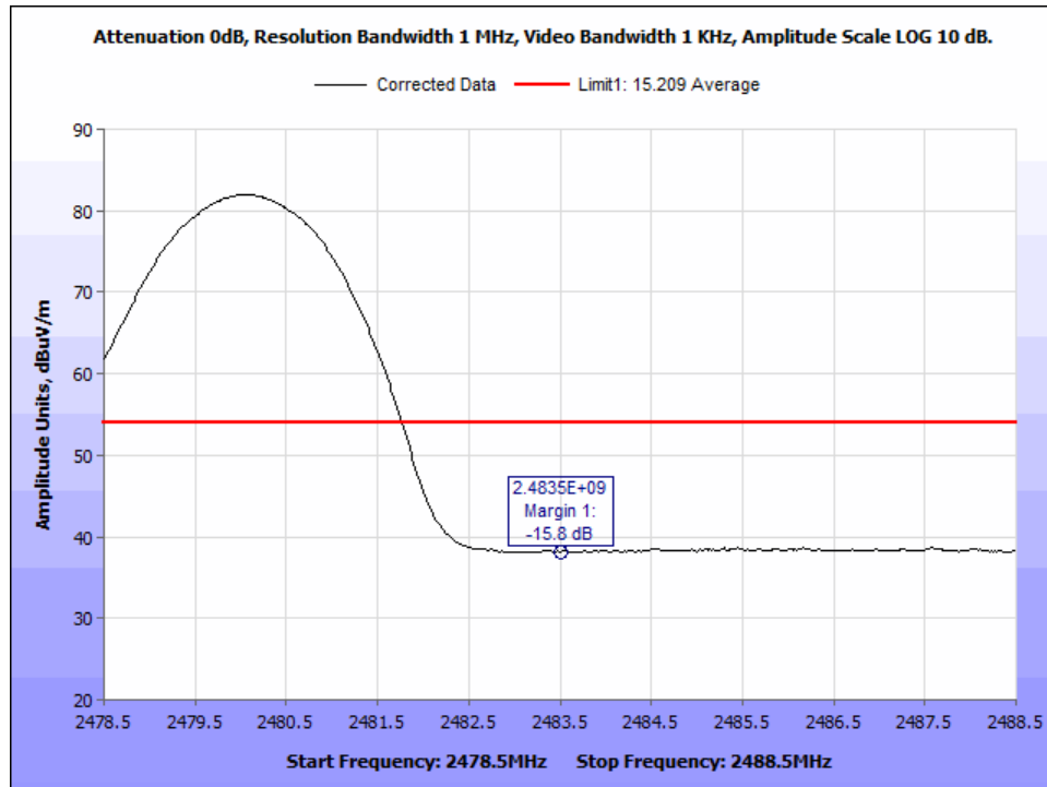
Figure 22: Average Radiated Bandedge @2483.5MHz – pi/4 DQPSK 2480MHz.
