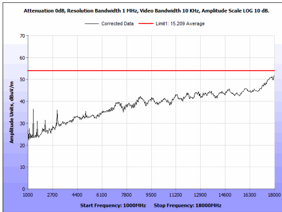
Figure 10: 15.209 Average Radiated Emissions - GFSK 2402MHz - 1-18GHz.
