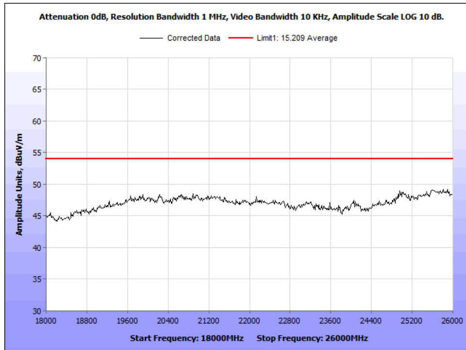
Figure 12: Radiated Emissions, Average, 18 GHz – 26 GHz
