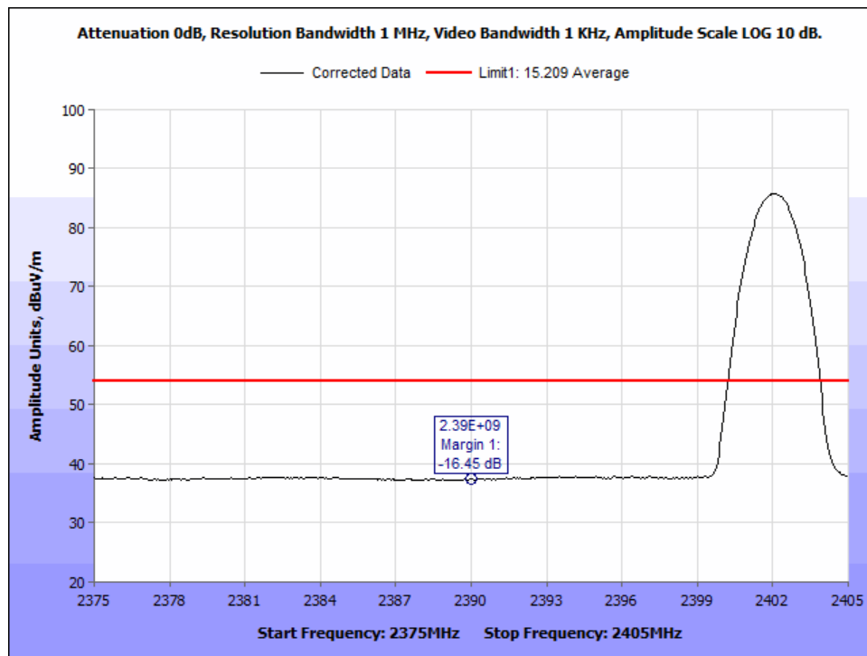
Figure 17: Average Radiated Bandedge @2390MHz - 8DPSK 2402MHz.
