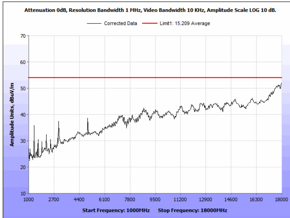
Figure 11: 15.209 Average Radiated Emissions - GFSK 2480MHz - 1-18GHz.
