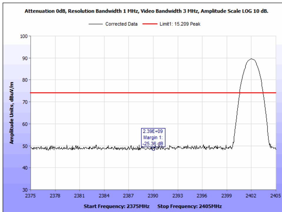
Figure 23: Peak Radiated Bandedge @2390MHz - 8DPSK 2402MHz.
