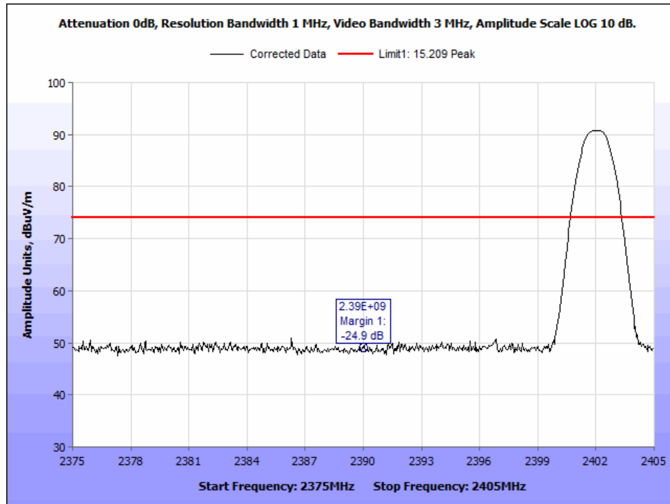
Figure 24: Peak Radiated Bandedge @2390MHz - GFSK 2402MHz.
