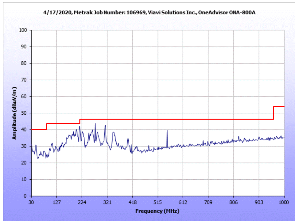
Figure 16: Radiated Emissions, Worst Case, 30-1000MHz
