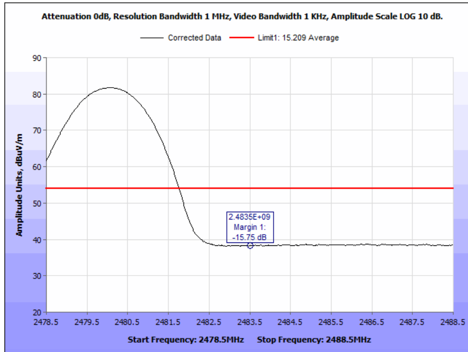
Figure 20: Average Radiated Bandedge @2483.5MHz - 8DPSK 2480MHz.
