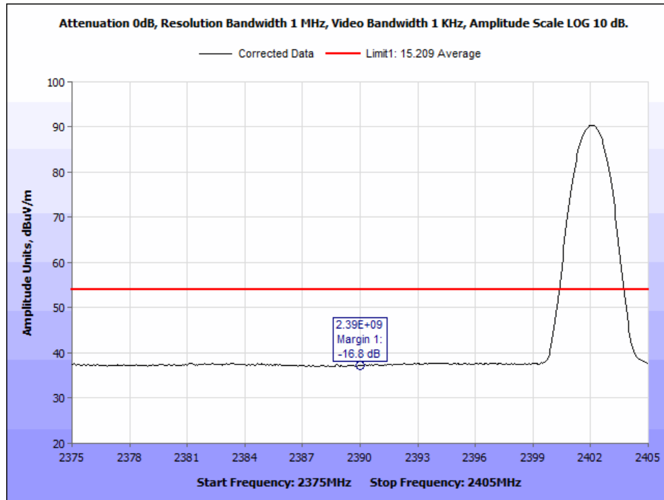
Figure 18: Average Radiated Bandedge @2390MHz - GFSK 2402MHz.
