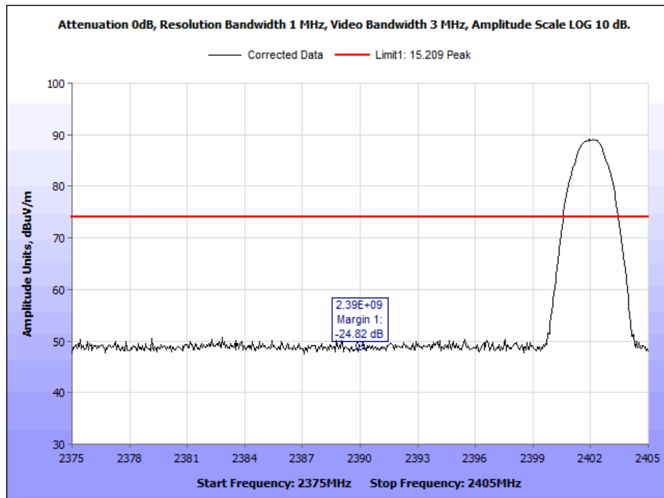
Figure 25: Peak Radiated Bandedge @2390MHz – pi/4 DQPSK 2402MHz.
