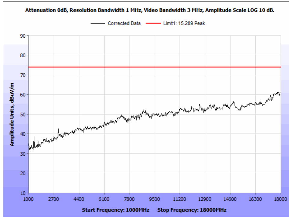
Figure 13: 15.209 Peak Radiated Emissions - GFSK 2402MHz - 1-18GHz.
