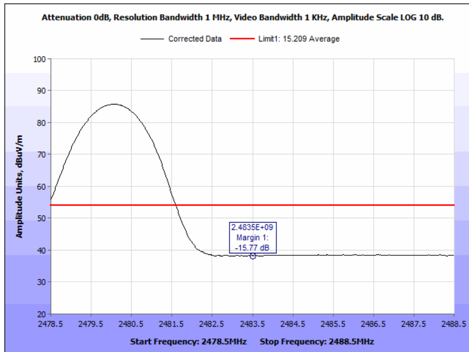
Figure 21: Average Radiated Bandedge @2483.5MHz - GFSK 2480MHz.
