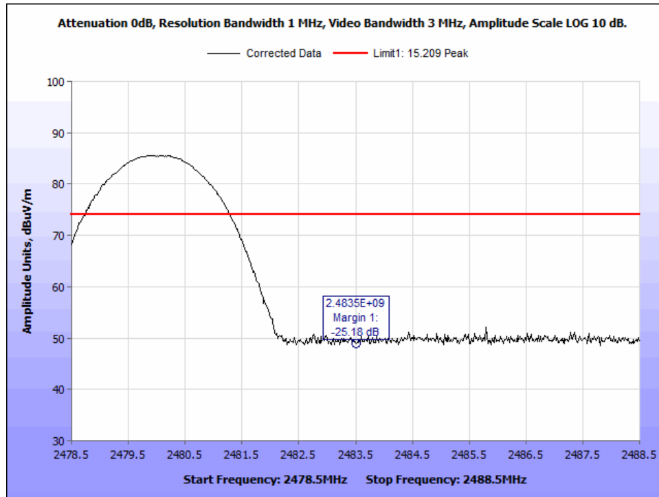
Figure 28: Peak Radiated Bandedge @2483.5MHz – pi/4 DQPSK 2480MHz.
