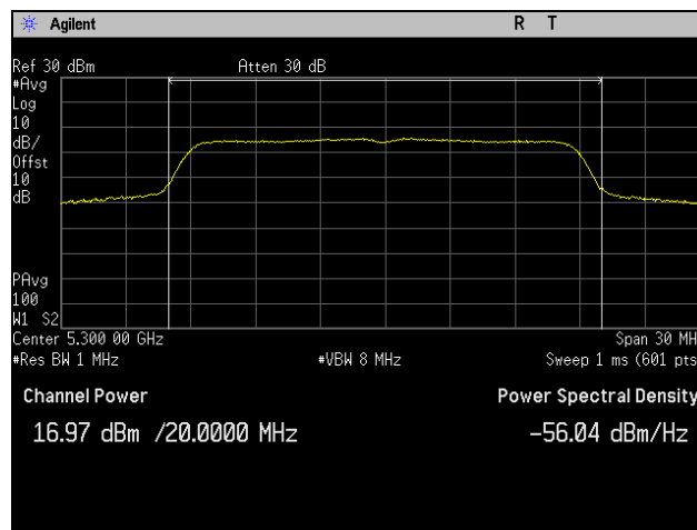
Plot 181. Maximum Conducted Output Power, 802.11ac 20 MHz, Channel 5300 MHz, 2SS, P1
