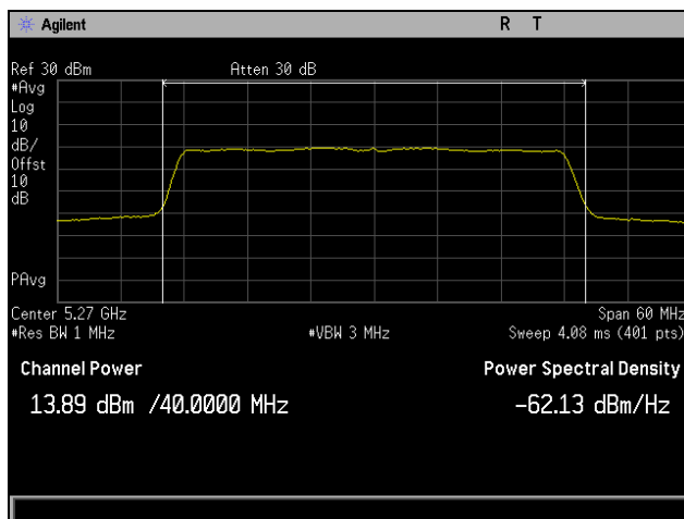
Plot 335. Maximum Conducted Output Power, 802.11n 40 MHz, Channel 5270 MHz, 3SS, P2
