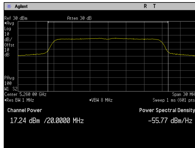
Plot 276. Maximum Conducted Output Power, 802.11n 20 MHz, Channel 5260 MHz, 2SS, P1
