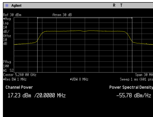
Plot 173. Maximum Conducted Output Power, 802.11ac 20 MHz, Channel 5260 MHz, 1SS
