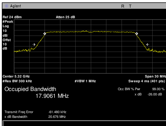
Plot 126. Occupied Bandwidth, 802.11n 20 MHz, Channel 5320 MHz, 3SS, P3, 26 dB
