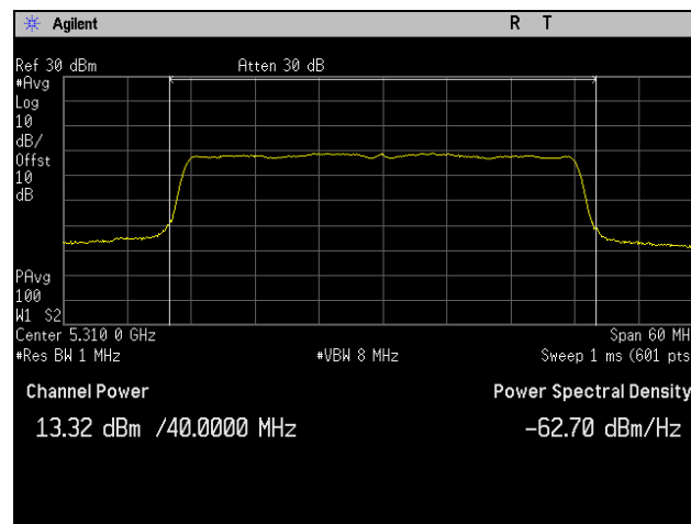
Plot 324. Maximum Conducted Output Power, 802.11n 40 MHz, Channel 5310 MHz, 2SS, P2
