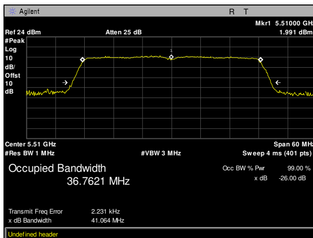
Plot 162. Occupied Bandwidth, 802.11n 40 MHz, Channel 5510 MHz, 3SS, P3, 26 dB
