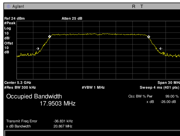
Plot 107. Occupied Bandwidth, 802.11n 20 MHz, Channel 5300 MHz, 2SS, P2, 26 dB
