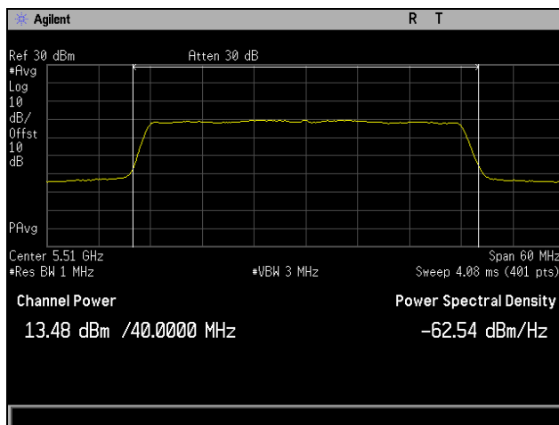
Plot 337. Maximum Conducted Output Power, 802.11n 40 MHz, Channel 5510 MHz, 3SS, P2
