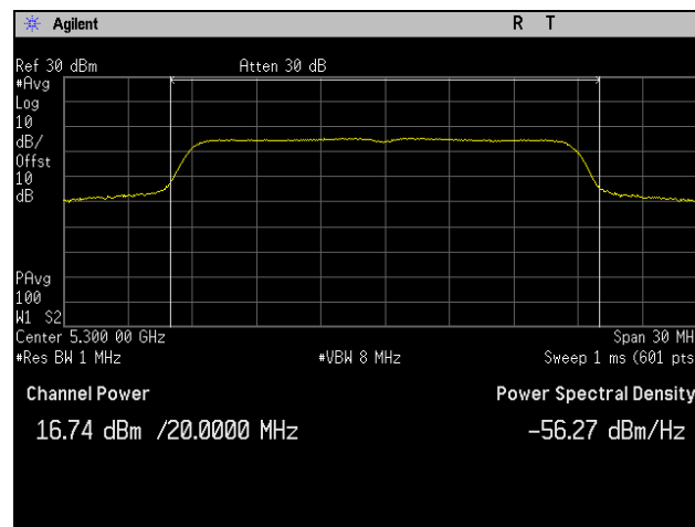
Plot 277. Maximum Conducted Output Power, 802.11n 20 MHz, Channel 5300 MHz, 2SS, P1
