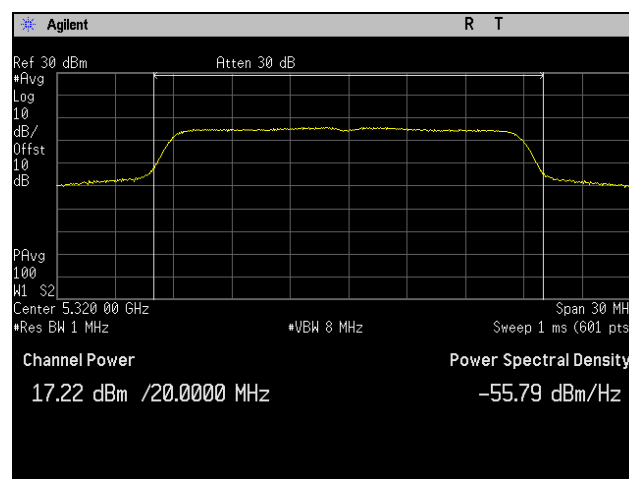
Plot 175. Maximum Conducted Output Power, 802.11ac 20 MHz, Channel 5320 MHz, 1SS
