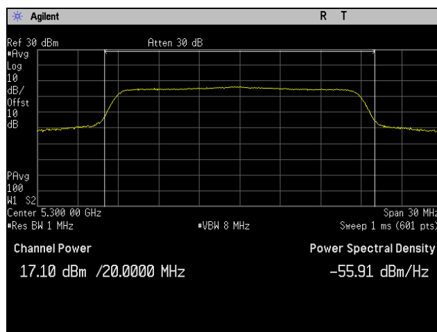
Plot 188. Maximum Conducted Output Power, 802.11ac 20 MHz, Channel 5300 MHz, 2SS, P2
