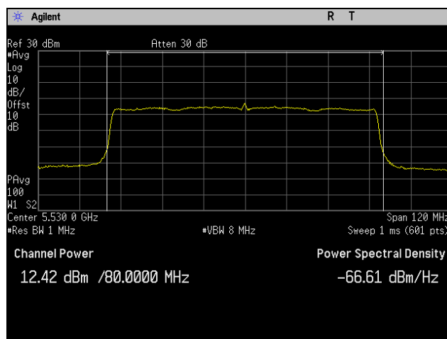
Plot 258. Maximum Conducted Output Power, 802.11ac 80 MHz, Channel 5530 MHz, 2SS, P2
