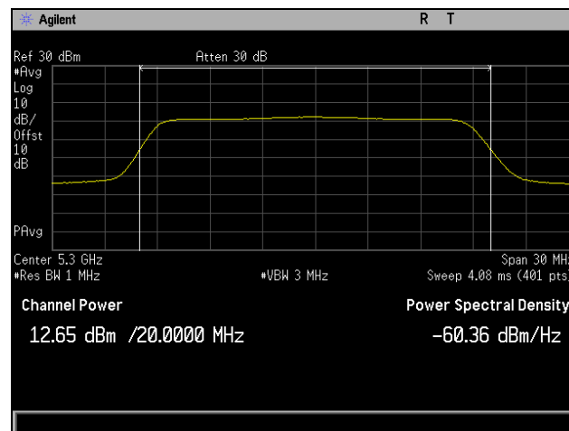
Plot 298. Maximum Conducted Output Power, 802.11n 20 MHz, Channel 5300 MHz, 3SS, P2
