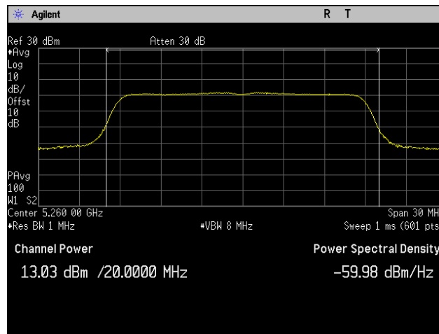
Plot 180. Maximum Conducted Output Power, 802.11ac 20 MHz, Channel 5260 MHz, 2SS, P1
