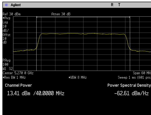
Plot 239. Maximum Conducted Output Power, 802.11ac 40 MHz, Channel 5270 MHz, 3SS, P2
