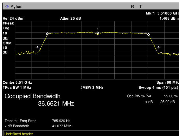
Plot 63. Occupied Bandwidth, 802.11ac 40 MHz, Channel 5510 MHz, 3SS, P1, 26 dB
