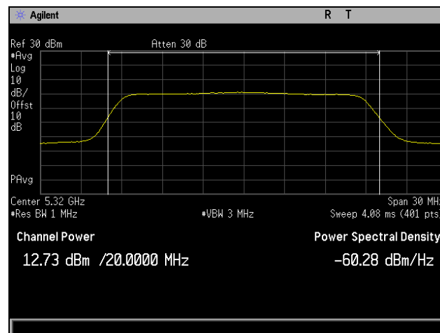
Plot 299. Maximum Conducted Output Power, 802.11n 20 MHz, Channel 5320 MHz, 3SS, P2
