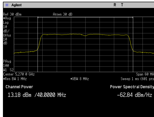
Plot 245. Maximum Conducted Output Power, 802.11ac 40 MHz, Channel 5270 MHz, 3SS, P3
