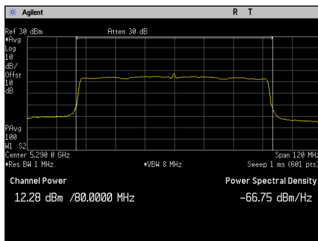
Plot 257. Maximum Conducted Output Power, 802.11ac 80 MHz, Channel 5290 MHz, 2SS, P2
