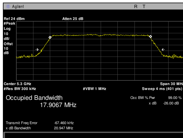
Plot 95. Occupied Bandwidth, 802.11n 20 MHz, Channel 5300 MHz, 1SS, 26 dB
