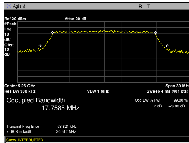
Plot 106. Occupied Bandwidth, 802.11n 20 MHz, Channel 5260 MHz, 2SS, P2, 26 dB
