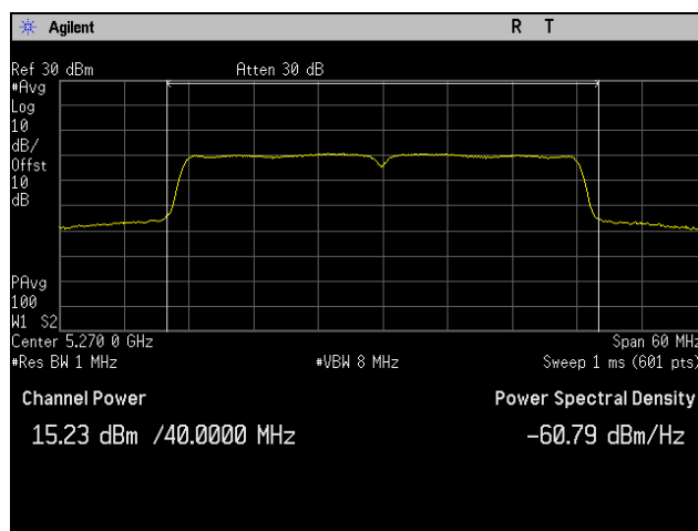
Plot 215. Maximum Conducted Output Power, 802.11ac 40 MHz, Channel 5270 MHz, 1SS
