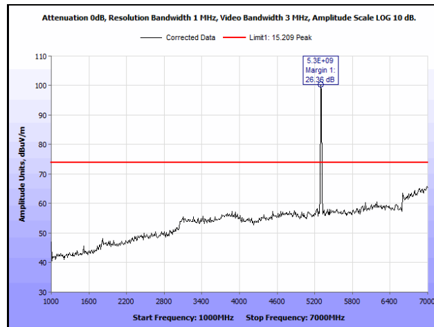
Plot 566. Radiated Spurious Emissions, 802.11ac 20 MHz, Channel 60, 1SS, 1 GHz – 7 GHz, Peak
