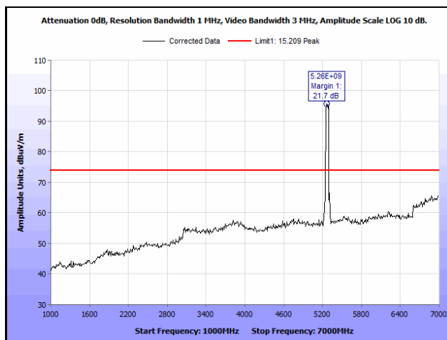
Plot 886. Radiated Spurious Emissions, 802.11n 40 MH, Channel 54, 2SS, 1 GHz – 7 GHz, Peak
