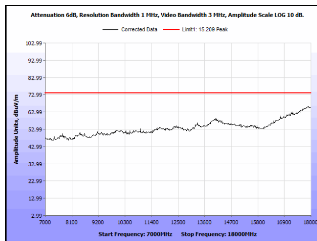
Plot 558. Radiated Spurious Emissions, 802.11a 20 MHz, Channel 144, 7 GHz – 18 GHz, Peak
