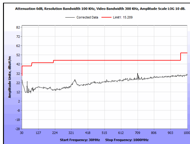
Plot 534. Radiated Spurious Emissions, 802.11a 20 MHz, Channel 60, 30 MHz – 1 GHz
