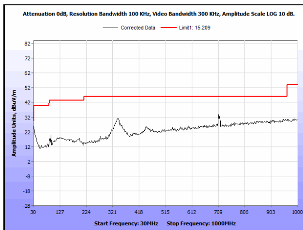
Plot 549. Radiated Spurious Emissions, 802.11a 20 MH, Channel 116, 30 MHz – 1 GHz
