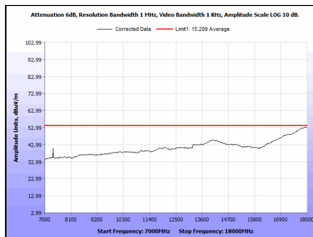
Plot 612. Radiated Spurious Emissions, 802.11ac 20 MHz, Channel 116, 2SS, 7 GHz – 18 GHz, Average
