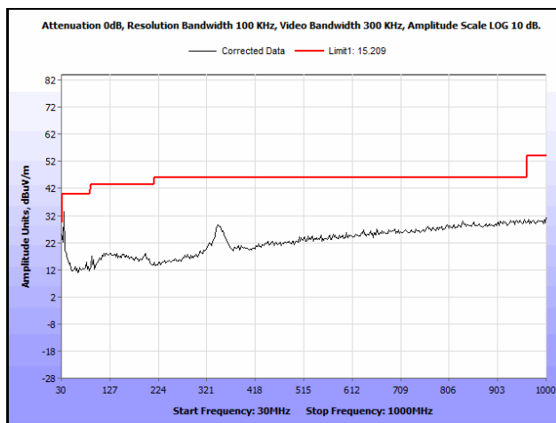
Plot 759. Radiated Spurious Emissions, 802.11ac 80 MH, Channel 106, 3SS, 30 MHz – 1 GHz
