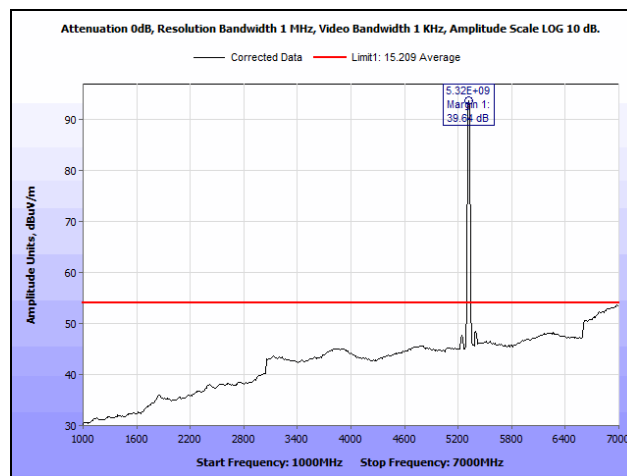
Plot 810. Radiated Spurious Emissions, 802.11n 20 MHz, Channel 64, 2SS, 1 GHz – 7 GHz, Average
