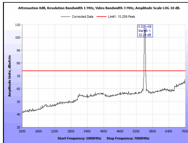
Plot 661. Radiated Spurious Emissions, 802.11ac 40 MHz, Channel 102, 1SS, 1 GHz – 7 GHz, Peak
