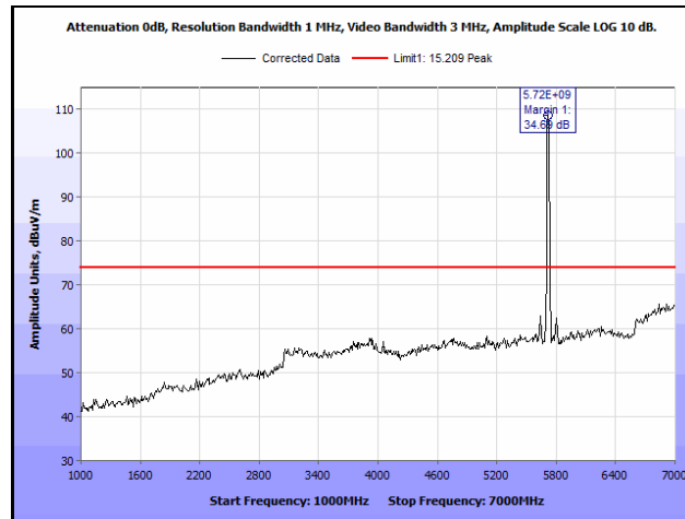
Plot 826. Radiated Spurious Emissions, 802.11n 20 MHz, Channel 144, 2SS, 1 GHz – 7 GHz, Peak
