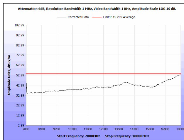
Plot 822. Radiated Spurious Emissions, 802.11n 20 MH, Channel 116, 2SS, 7 GHz – 18 GHz, Average
