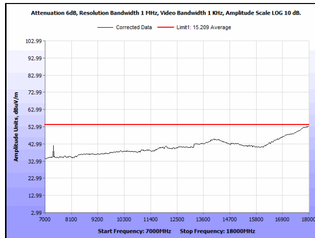
Plot 897. Radiated Spurious Emissions, 802.11n 40 MHz, Channel 102, 2SS, 7 GHz – 18 GHz, Average
