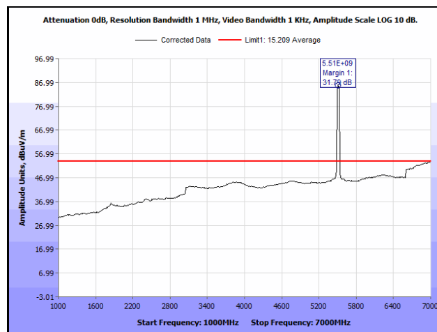
Plot 870. Radiated Spurious Emissions, 802.11n 40 MHz, Channel 102, 1SS, 1 GHz – 7 GHz, Average
