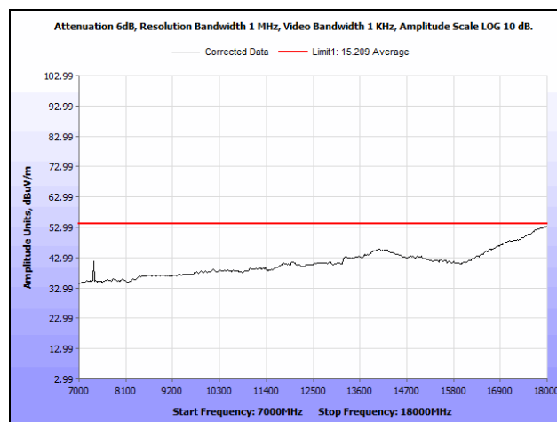
Plot 932. Radiated Spurious Emissions, 802.11n 40 MH, Channel 142, 3SS, 7 GHz – 18 GHz, Average
