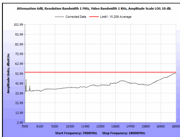
Plot 712. Radiated Spurious Emissions, 802.11ac 40 MHz, Channel 102, 3SS, 7 GHz – 18 GHz, Average
