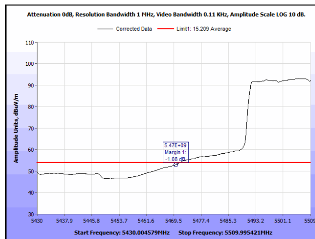
Plot 1014. Radiated Band Edge, 802.11n 40 MHz, 2SS, 5470 MHz, Average
