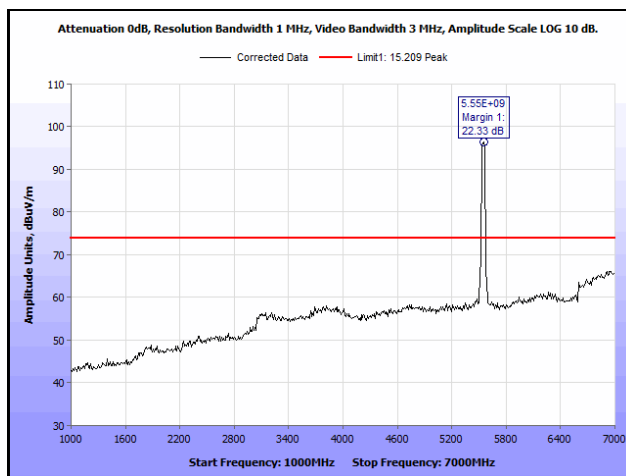
Plot 876. Radiated Spurious Emissions, 802.11n 40 MHz, Channel 110, 1SS, 1 GHz – 7 GHz, Peak
