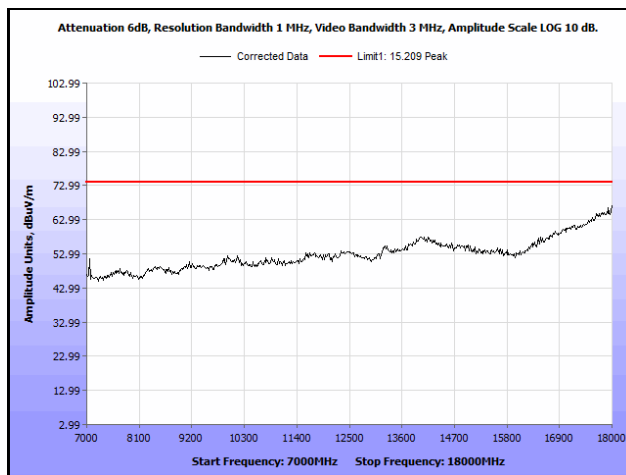
Plot 758. Radiated Spurious Emissions, 802.11ac 80 MH, Channel 58, 3SS, 7 GHz – 18 GHz, Peak
