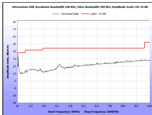
Plot 774. Radiated Spurious Emissions, 802.11n 20 MH, Channel 60, 1SS, 30 MHz – 1 GHz
