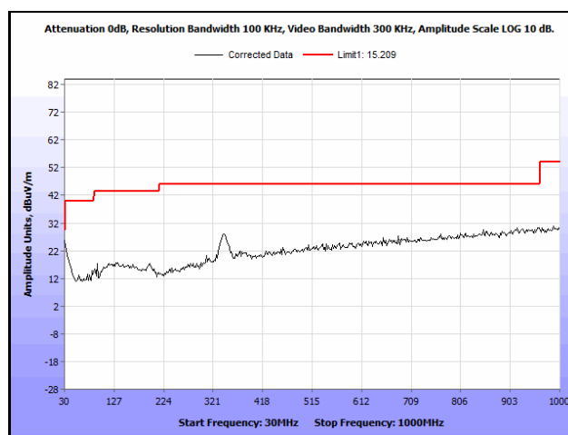
Plot 849. Radiated Spurious Emissions, 802.11n 20 MH, Channel 116, 3SS, 30 MHz – 1 GHz
