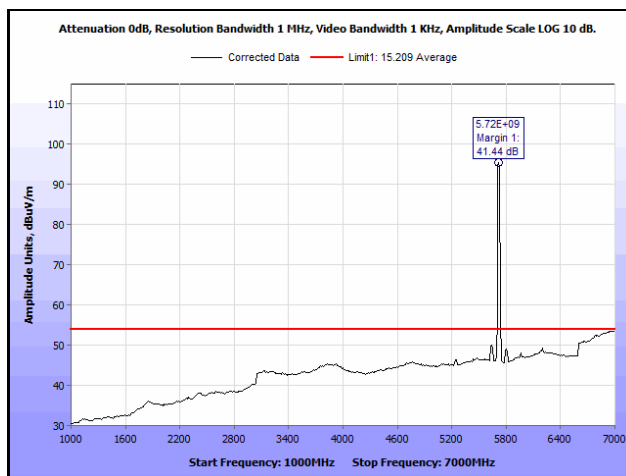
Plot 825. Radiated Spurious Emissions, 802.11n 20 MHz, Channel 144, 2SS, 1 GHz – 7 GHz, Average
