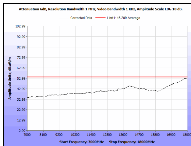
Plot 792. Radiated Spurious Emissions, 802.11n 20 MH, Channel 116, 1SS, 7 GHz – 18 GHz, Average
