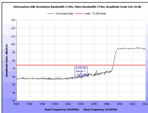
Plot 961. Radiated Band Edge, 802.11ac 40 MHz, 1SS, 5470 MHz, Peak
