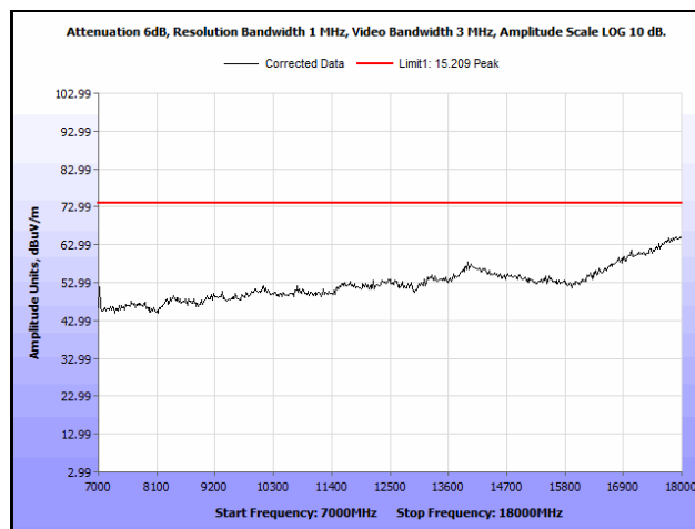
Plot 893. Radiated Spurious Emissions, 802.11n 40 MHz, Channel 62, 2SS, 7 GHz – 18 GHz, Peak
