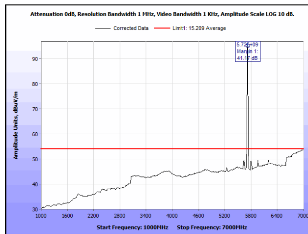
Plot 585. Radiated Spurious Emissions, 802.11ac 20 MHz, Channel 144, 1SS, 1 GHz – 7 GHz, Average
