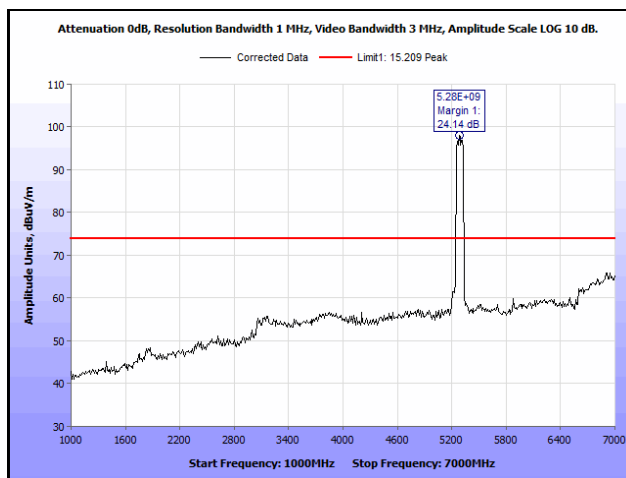
Plot 756. Radiated Spurious Emissions, 802.11ac 80 MHz, Channel 58, 3SS, 1 GHz – 7 GHz, Peak
