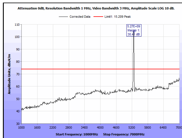
Plot 801. Radiated Spurious Emissions, 802.11n 20 MHz, Channel 52, 2SS, 1 GHz – 7 GHz, Peak
