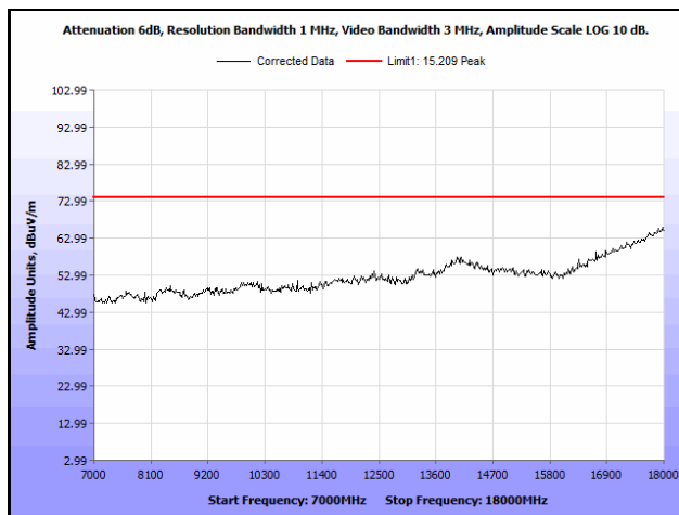
Plot 548. Radiated Spurious Emissions, 802.11a 20 MH, Channel 100, 7 GHz – 18 GHz, Peak
