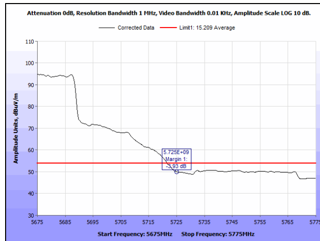
Plot 968. Radiated Band Edge, 802.11ac 40 MHz, 2SS, 5725 MHz, Average
