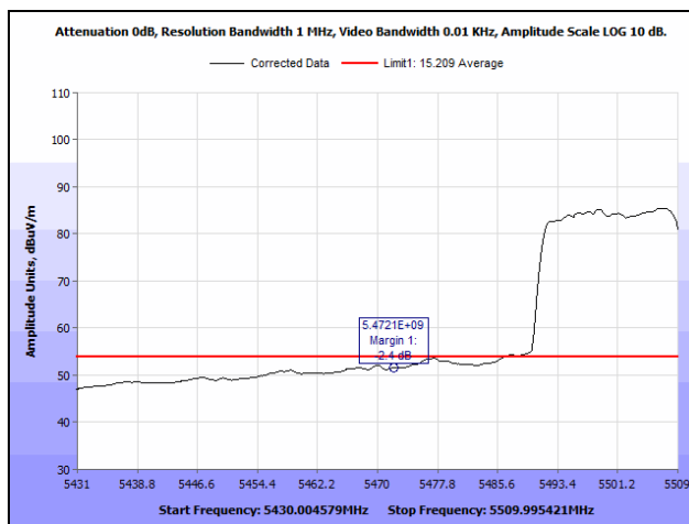
Plot 986. Radiated Band Edge, 802.11ac 80 MHz, 3SS, 5470 MHz, Average
