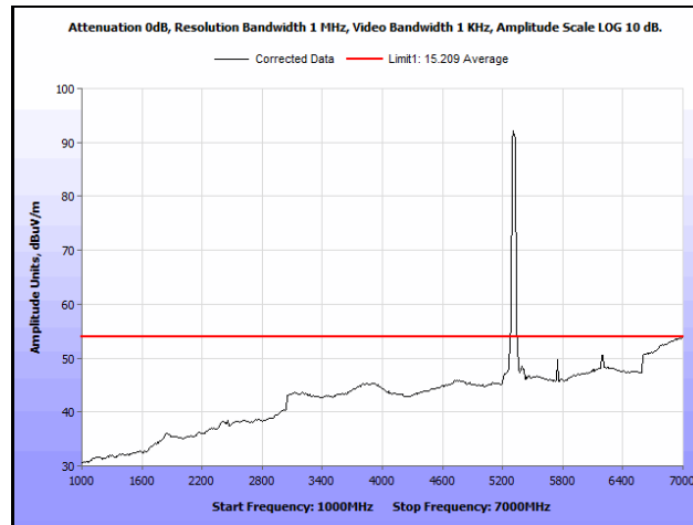
Plot 680. Radiated Spurious Emissions, 802.11ac 40 MHz, Channel 62, 2SS, 1 GHz – 7 GHz, Average
