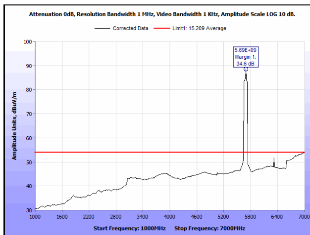
Plot 750. Radiated Spurious Emissions, 802.11ac 80 MHz, Channel 138, 2SS, 1 GHz – 7 GHz, Average
