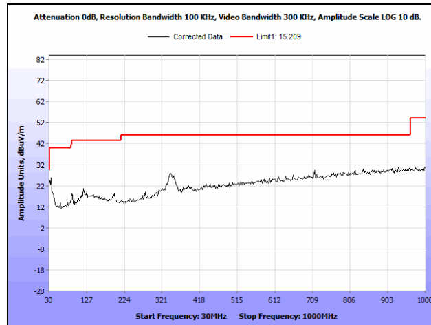
Plot 809. Radiated Spurious Emissions, 802.11n 20 MHz, Channel 64, 2SS, 30 MHz – 1 GHz
