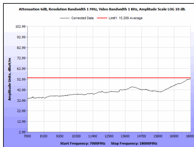
Plot 732. Radiated Spurious Emissions, 802.11ac 80 MHz, Channel 106, 1SS, 7 GHz – 18 GHz, Average
