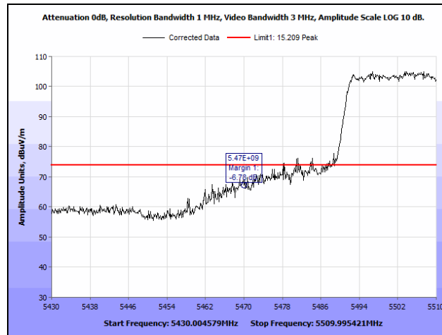
Plot 967. Radiated Band Edge, 802.11ac 40 MHz, 2SS, 5470 MHz, Peak
