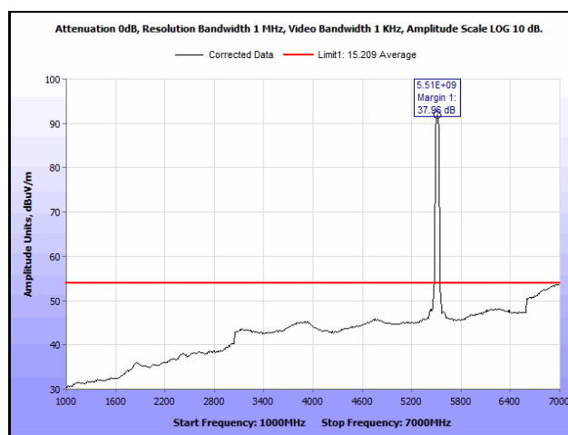
Plot 895. Radiated Spurious Emissions, 802.11n 40 MHz, Channel 102, 2SS, 1 GHz – 7 GHz, Average
