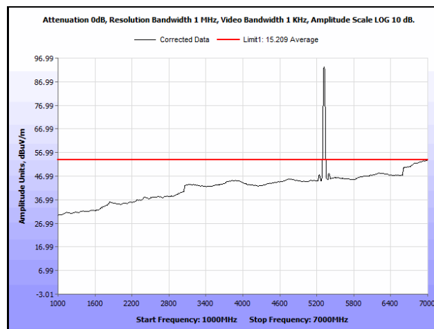
Plot 540. Radiated Spurious Emissions, 802.11a 20 MHz, Channel 64, 1 GHz – 7 GHz, Average
