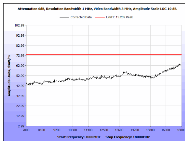
Plot 848. Radiated Spurious Emissions, 802.11n 20 MH, Channel 100, 3SS, 7 GHz – 18 GHz, Peak
