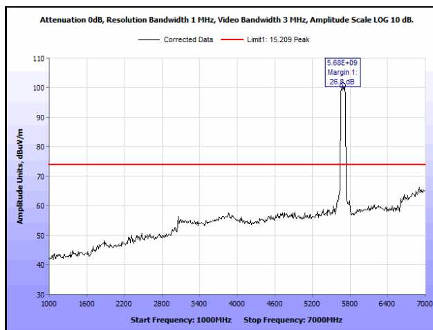
Plot 766. Radiated Spurious Emissions, 802.11ac 80 MHz, Channel 138, 3SS, 1 GHz – 7 GHz, Peak
