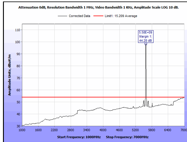
Plot 610. Radiated Spurious Emissions, 802.11ac 20 MHz, Channel 116, 2SS, 1 GHz – 7 GHz, Average
