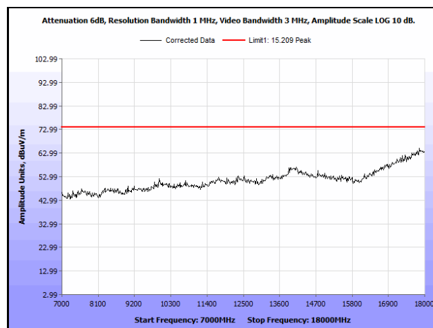
Plot 843. Radiated Spurious Emissions, 802.11n 20 MH, Channel 64, 3SS, 7 GHz – 18 GHz, Peak
