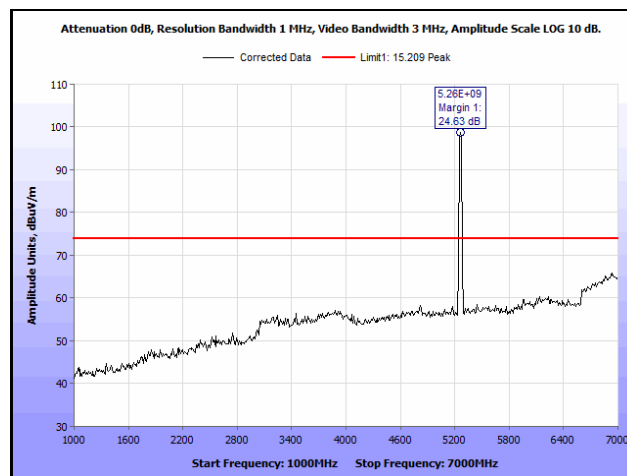
Plot 561. Radiated Spurious Emissions, 802.11ac 20 MHz, Channel 52, 1SS, 1 GHz – 7 GHz, Peak
