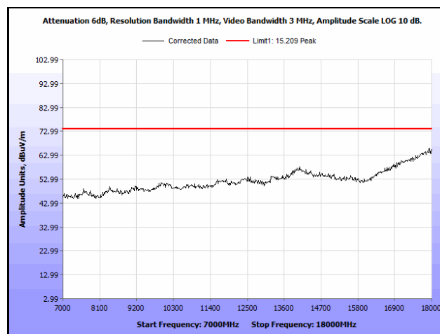
Plot 633. Radiated Spurious Emissions, 802.11ac 20 MHz, Channel 64, 3SS, 7 GHz – 18 GHz, Peak
