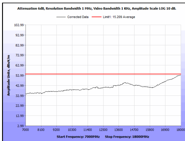
Plot 547. Radiated Spurious Emissions, 802.11a 20 MH, Channel 100, 7 GHz – 18 GHz, Average
