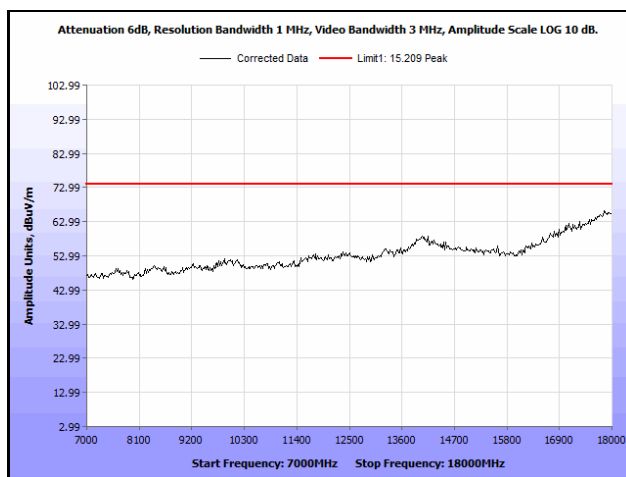
Plot 543. Radiated Spurious Emissions, 802.11a 20 MH, Channel 64, 7 GHz – 18 GHz, Peak
