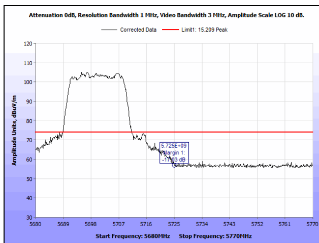
Plot 957. Radiated Band Edge, 802.11ac 20 MHz, 3SS, 5725 MHz, Peak
