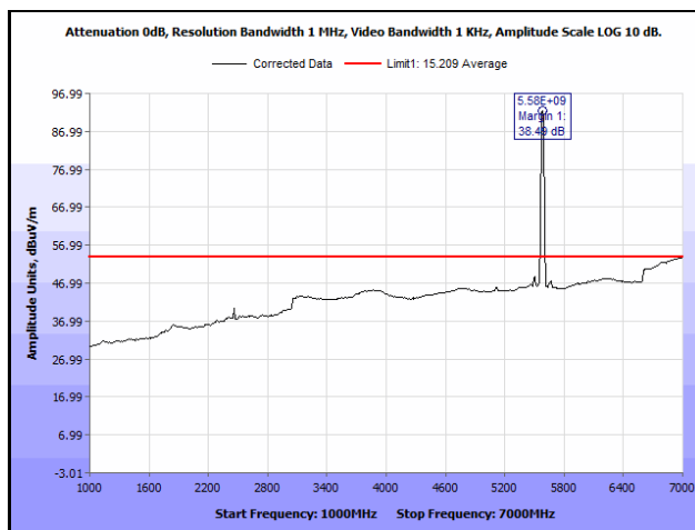
Plot 550. Radiated Spurious Emissions, 802.11a 20 MHz, Channel 116, 1 GHz – 7 GHz, Average
