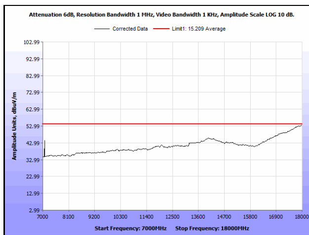
Plot 587. Radiated Spurious Emissions, 802.11ac 20 MHz, Channel 144, 1SS, 7 GHz – 18 GHz, Average
