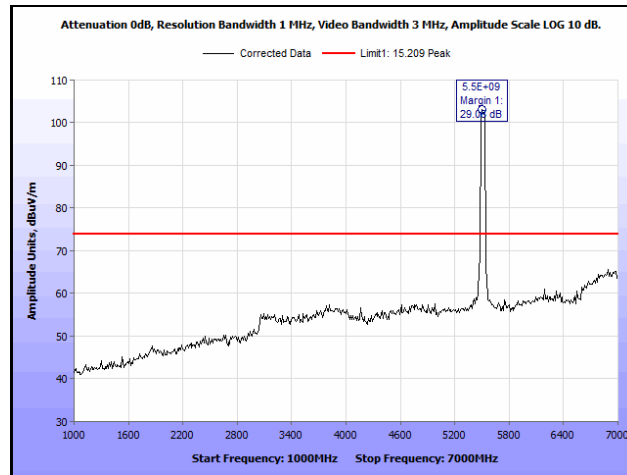
Plot 921. Radiated Spurious Emissions, 802.11n 40 MHz, Channel 102, 3SS, 1 GHz – 7 GHz, Peak
