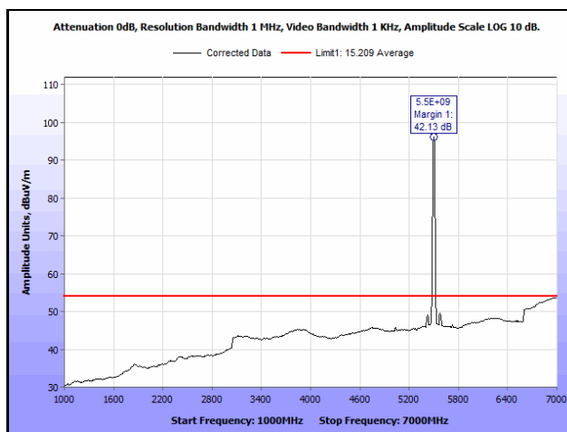
Plot 845. Radiated Spurious Emissions, 802.11n 20 MHz, Channel 100, 3SS, 1 GHz – 7 GHz, Average
