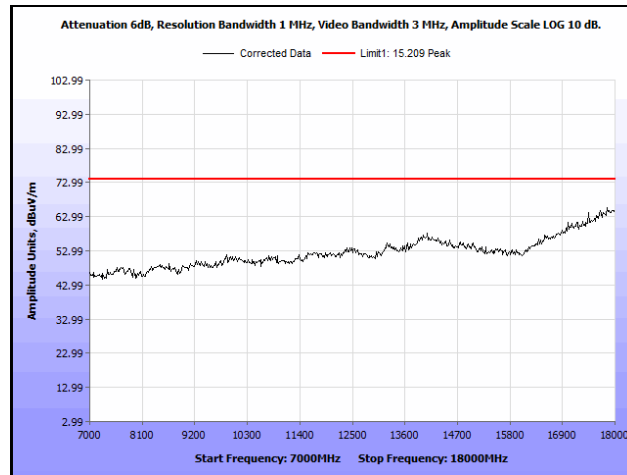
Plot 793. Radiated Spurious Emissions, 802.11n 20 MHz, Channel 116, 1SS, 7 GHz – 18 GHz, Peak
