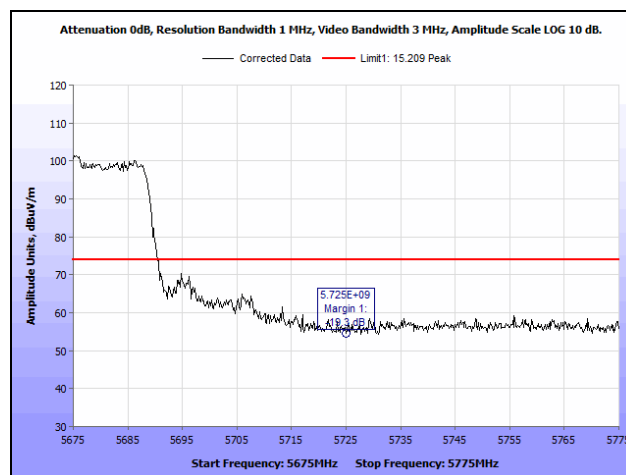
Plot 1023. Radiated Band Edge, 802.11n 40 MHz, 3SS, 5725 MHz, Peak
