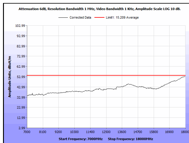
Plot 762. Radiated Spurious Emissions, 802.11ac 80 MHz, Channel 106, 3SS, 7 GHz – 18 GHz, Average
