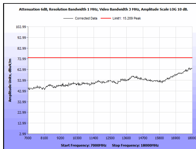
Plot 798. Radiated Spurious Emissions, 802.11n 20 MHz, Channel 144, 1SS, 7 GHz – 18 GHz, Peak
