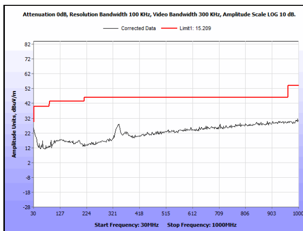
Plot 919. Radiated Spurious Emissions, 802.11n 40 MHz, Channel 102, 3SS, 30 MHz – 1 GHz
