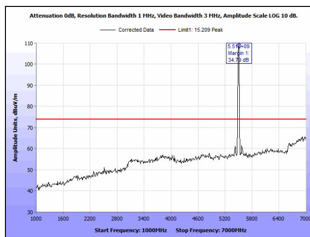
Plot 816. Radiated Spurious Emissions, 802.11n 20 MHz, Channel 100, 2SS, 1 GHz – 7 GHz, Peak
