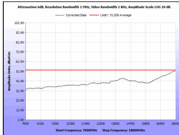
Plot 532. Radiated Spurious Emissions, 802.11a 20 MHz, Channel 52, 7 GHz – 18 GHz, Average
