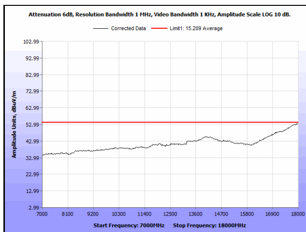
Plot 672. Radiated Spurious Emissions, 802.11ac 40 MH, Channel 142, 1SS, 7 GHz – 18 GHz, Average
