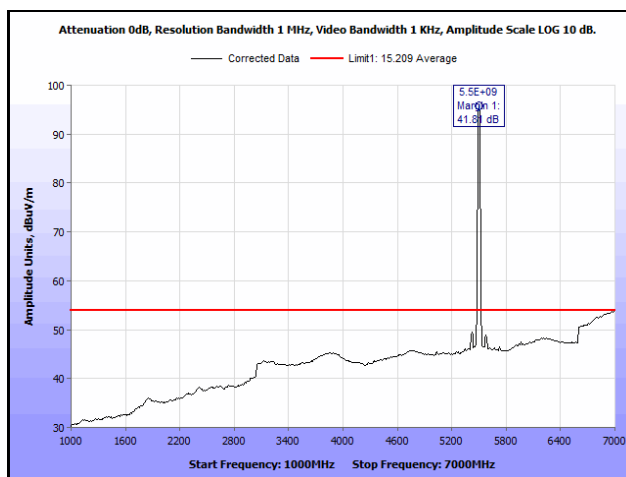
Plot 575. Radiated Spurious Emissions, 802.11ac 20 MHz, Channel 100, 1SS, 1 GHz – 7 GHz, Average
