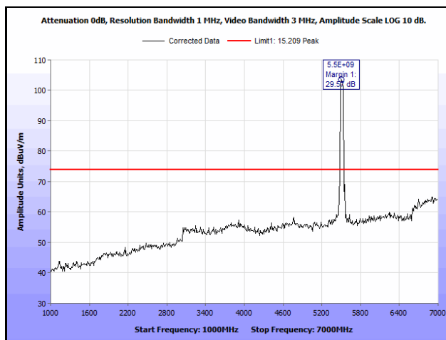
Plot 711. Radiated Spurious Emissions, 802.11ac 40 MHz, Channel 102, 3SS, 1 GHz – 7 GHz, Peak
