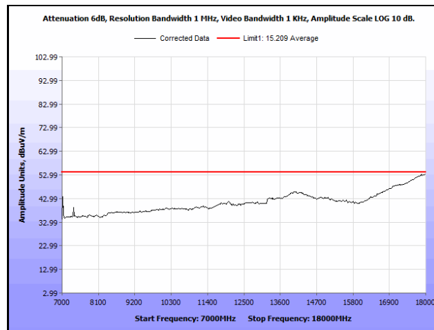
Plot 877. Radiated Spurious Emissions, 802.11n 40 MH, Channel 110, 1SS, 7 GHz – 18 GHz, Average
