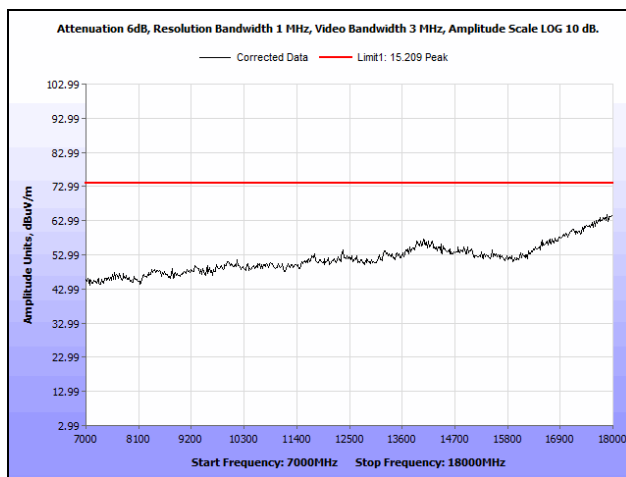
Plot 823. Radiated Spurious Emissions, 802.11n 20 MHz, Channel 116, 2SS, 7 GHz – 18 GHz, Peak
