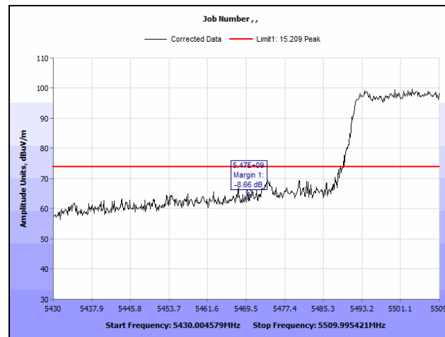
Plot 983. Radiated Band Edge, 802.11ac 80 MHz, 2SS, 5470 MHz, Peak
