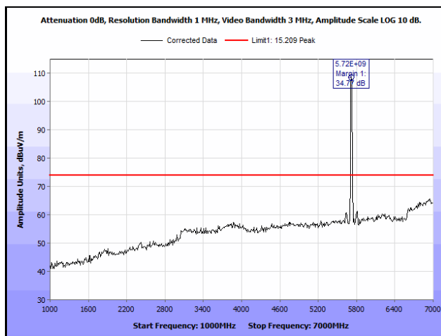
Plot 586. Radiated Spurious Emissions, 802.11ac 20 MHz, Channel 144, 1SS, 1 GHz – 7 GHz, Peak
