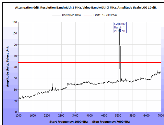
Plot 531. Radiated Spurious Emissions, 802.11a 20 MH, Channel 52, 1 GHz – 7 GHz, Peak
