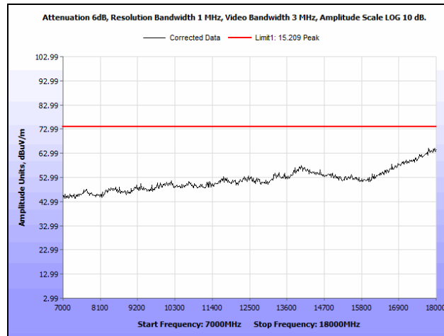
Plot 808. Radiated Spurious Emissions, 802.11n 20 MHz, Channel 60, 2SS, 7 GHz – 18 GHz, Peak
