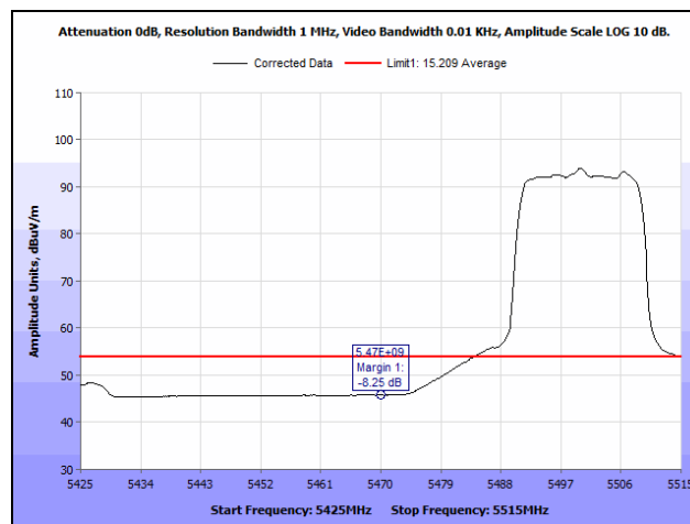
Plot 954. Radiated Band Edge, 802.11ac 20 MHz, 3SS, 5470 MHz, Average
