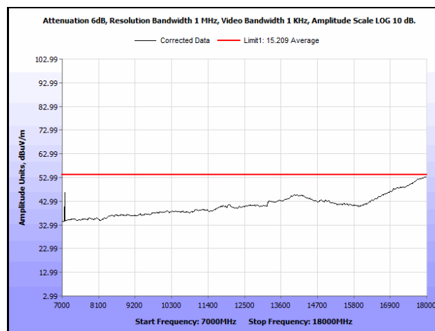
Plot 707. Radiated Spurious Emissions, 802.11ac 40 MHz, Channel 62, 3SS, 7 GHz – 18 GHz, Average
