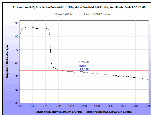
Plot 980. Radiated Band Edge, 802.11ac 80 MHz, 2SS, 5350 MHz, Average
