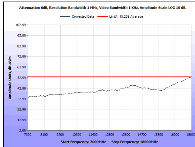
Plot 772. Radiated Spurious Emissions, 802.11n 20 MH, Channel 52, 1SS, 7 GHz – 18 GHz, Average
