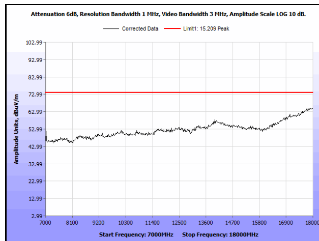
Plot 898. Radiated Spurious Emissions, 802.11n 40 MHz, Channel 102, 2SS, 7 GHz – 18 GHz, Peak
