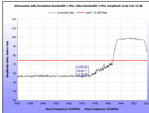
Plot 943. Radiated Band Edge, 802.11ac 20 MHz, 5470 MHz, Peak
