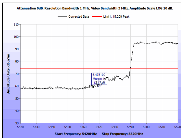
Plot 1009. Radiated Band Edge, 802.11n 40 MHz, 1SS, 5470 MHz, Peak
