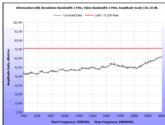
Plot 573. Radiated Spurious Emissions, 802.11ac 20 MHz, Channel 64, 1SS, 7 GHz – 18 GHz, Peak
