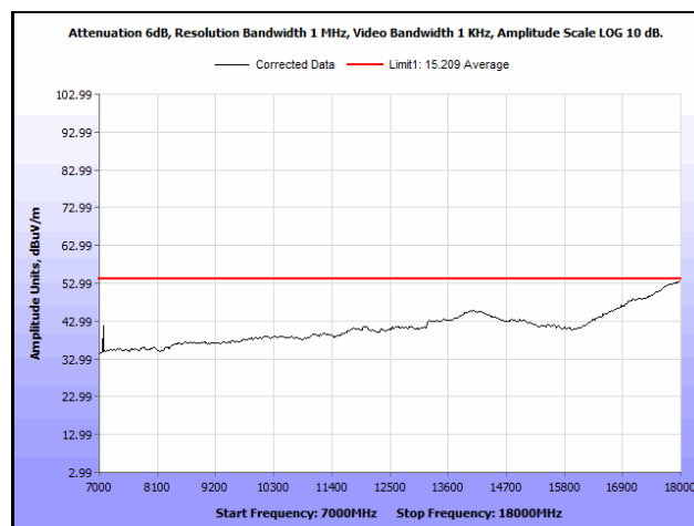
Plot 657. Radiated Spurious Emissions, 802.11ac 40 MHz, Channel 62, 1SS, 7 GHz – 18 GHz, Average
