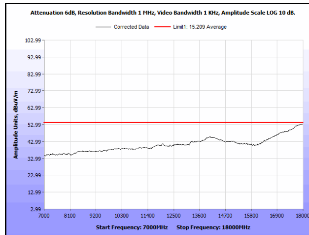
Plot 687. Radiated Spurious Emissions, 802.11ac 40 MHz, Channel 102, 2SS, 7 GHz – 18 GHz, Average
