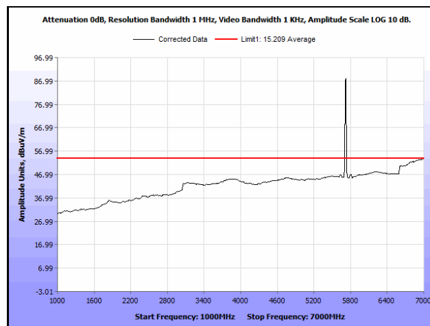
Plot 795. Radiated Spurious Emissions, 802.11n 20 MHz, Channel 144, 1SS, 1 GHz – 7 GHz, Average
