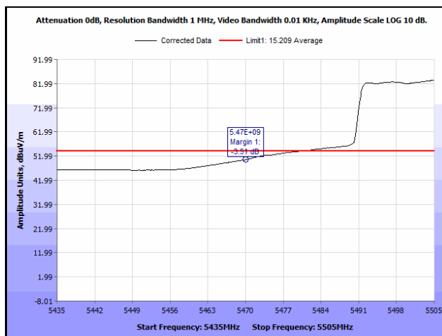
Plot 1008. Radiated Band Edge, 802.11n 40 MHz, 1SS, 5470 MHz, Average
