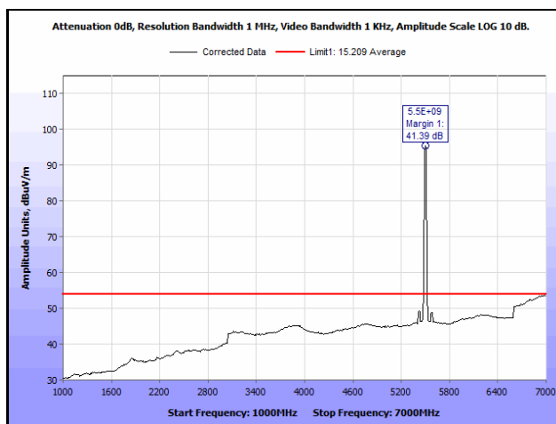
Plot 605. Radiated Spurious Emissions, 802.11ac 20 MHz, Channel 100, 2SS, 1 GHz – 7 GHz, Average
