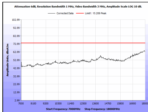
Plot 873. Radiated Spurious Emissions, 802.11n 40 MHz, Channel 102, 1SS, 7 GHz – 18 GHz, Peak
