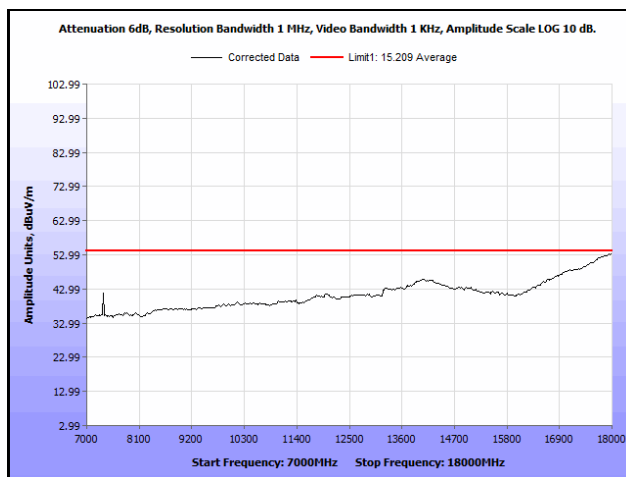
Plot 927. Radiated Spurious Emissions, 802.11n 40 MH, Channel 110, 3SS, 7 GHz – 18 GHz, Average
