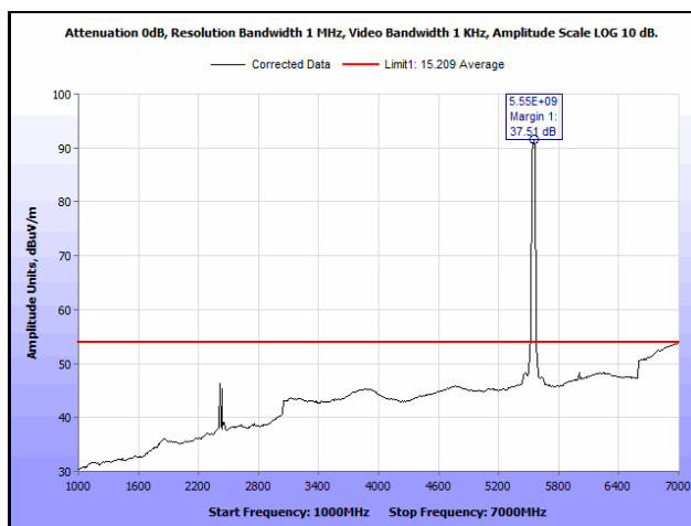
Plot 925. Radiated Spurious Emissions, 802.11n 40 MHz, Channel 110, 3SS, 1 GHz – 7 GHz, Average
