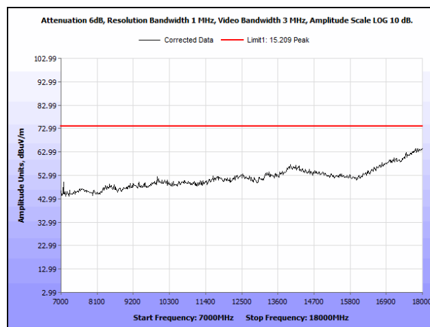
Plot 738. Radiated Spurious Emissions, 802.11ac 80 MHz, Channel 138, 1SS, 7 GHz – 18 GHz, Peak
