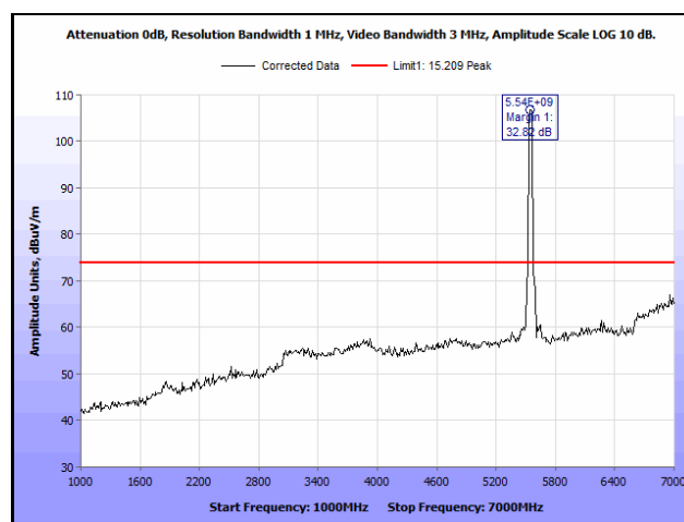
Plot 666. Radiated Spurious Emissions, 802.11ac 40 MHz, Channel 110, 1SS, 1 GHz – 7 GHz, Peak
