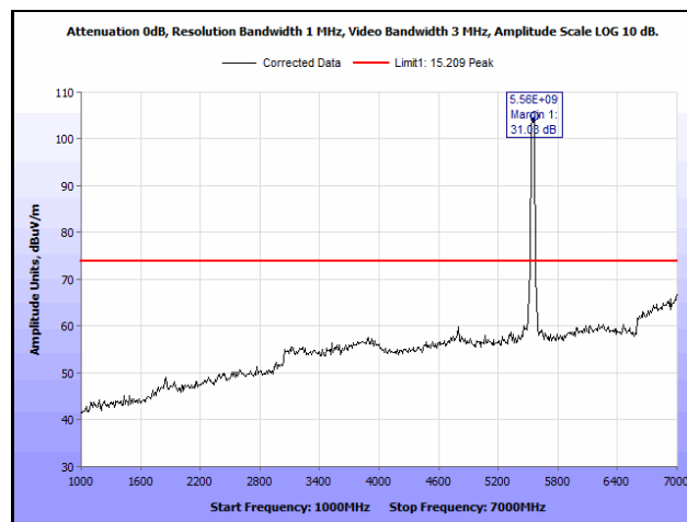
Plot 691. Radiated Spurious Emissions, 802.11ac 40 MHz, Channel 110, 2SS, 1 GHz – 7 GHz, Peak
