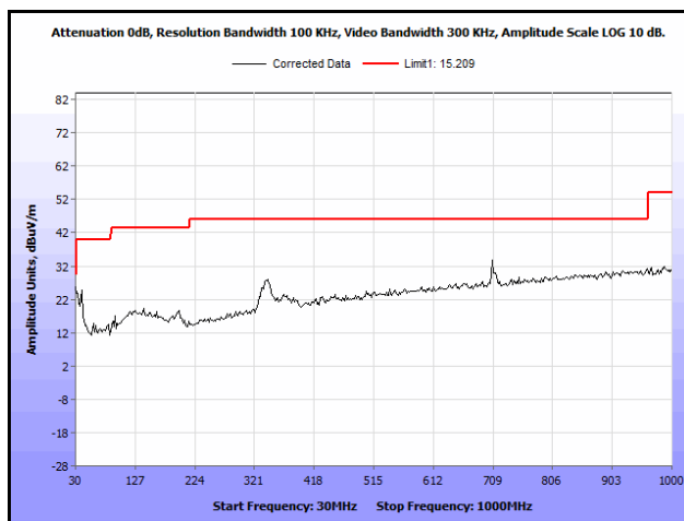
Plot 884. Radiated Spurious Emissions, 802.11n 40 MH, Channel 54, 2SS, 30 MHz – 1 GHz
