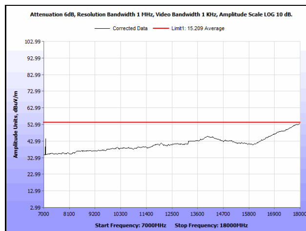
Plot 597. Radiated Spurious Emissions, 802.11ac 20 MHz, Channel 60, 2SS, 7 GHz – 18 GHz, Average
