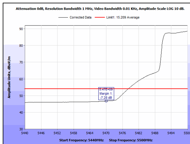
Plot 942. Radiated Band Edge, 802.11ac 20 MHz, 5470 MHz, Average
