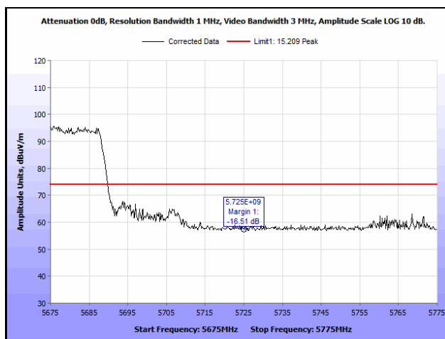
Plot 1011. Radiated Band Edge, 802.11n 40 MHz, 1SS, 5725 MHz, Peak
