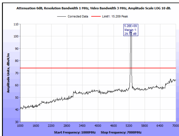
Plot 676. Radiated Spurious Emissions, 802.11ac 40 MHz, Channel 54, 2SS, 1 GHz – 7 GHz, Peak
