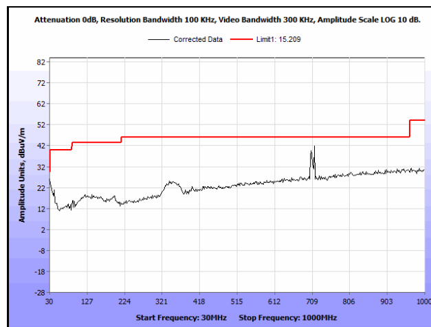
Plot 669. Radiated Spurious Emissions, 802.11ac 40 MH, Channel 142, 1SS, 30 MHz – 1 GHz
