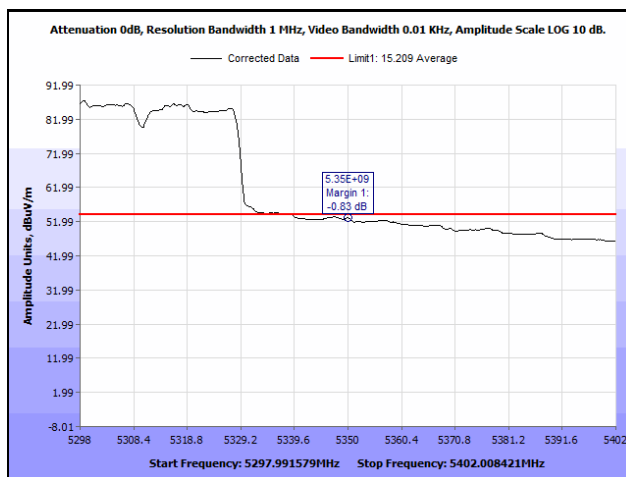
Plot 984. Radiated Band Edge, 802.11ac 80 MHz, 3SS, 5350 MHz, Average
