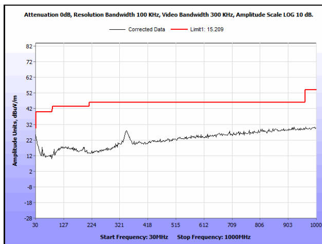
Plot 804. Radiated Spurious Emissions, 802.11n 20 MH, Channel 60, 2SS, 30 MHz – 1 GHz
