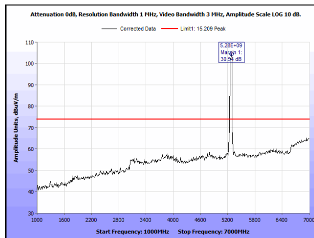
Plot 911. Radiated Spurious Emissions, 802.11n 40 MHz, Channel 54, 3SS, 1 GHz – 7 GHz, Peak
