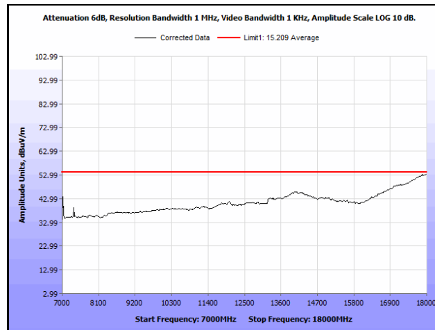
Plot 872. Radiated Spurious Emissions, 802.11n 40 MHz, Channel 102, 1SS, 7 GHz – 18 GHz, Average
