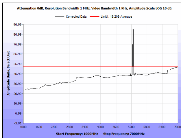
Plot 530. Radiated Spurious Emissions, 802.11a 20 MH, Channel 52, 1 GHz – 7 GHz, Average
