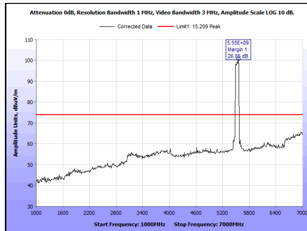
Plot 761. Radiated Spurious Emissions, 802.11ac 80 MHz, Channel 106, 3SS, 1 GHz – 7 GHz, Peak
