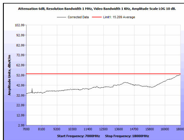
Plot 642. Radiated Spurious Emissions, 802.11ac 20 MHz, Channel 116, 3SS, 7 GHz – 18 GHz, Average
