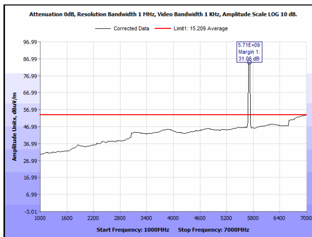
Plot 880. Radiated Spurious Emissions, 802.11n 40 MH, Channel 142, 1SS, 1 GHz – 7 GHz, Average
