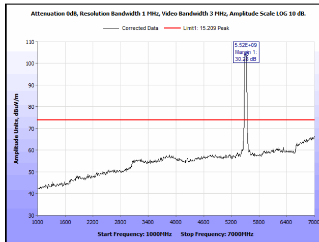
Plot 896. Radiated Spurious Emissions, 802.11n 40 MHz, Channel 102, 2SS, 1 GHz – 7 GHz, Peak
