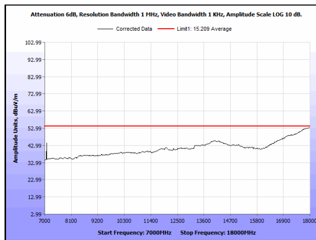
Plot 847. Radiated Spurious Emissions, 802.11n 20 MH, Channel 100, 3SS, 7 GHz – 18 GHz, Average
