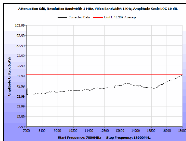
Plot 682. Radiated Spurious Emissions, 802.11ac 40 MHz, Channel 62, 2SS, 7 GHz – 18 GHz, Average
