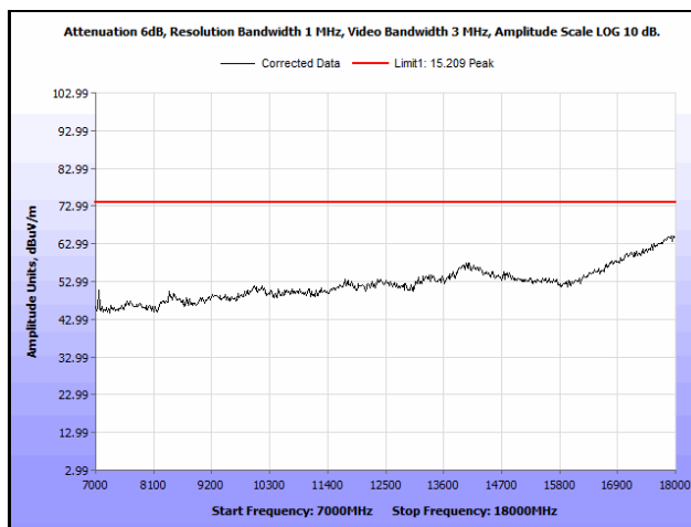
Plot 748. Radiated Spurious Emissions, 802.11ac 80 MHz, Channel 106, 2SS, 7 GHz – 18 GHz, Peak
