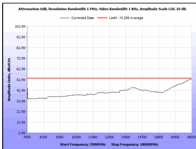
Plot 802. Radiated Spurious Emissions, 802.11n 20 MH, Channel 52, 2SS, 7 GHz – 18 GHz, Average
