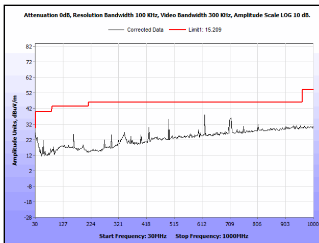
Plot 529. Radiated Spurious Emissions, 802.11a 20 MH, Channel 52, 30 MHz – 1 GHz
