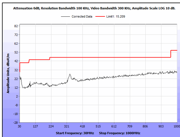
Plot 929. Radiated Spurious Emissions, 802.11n 40 MH, Channel 142, 3SS, 30 MHz – 1 GHz
