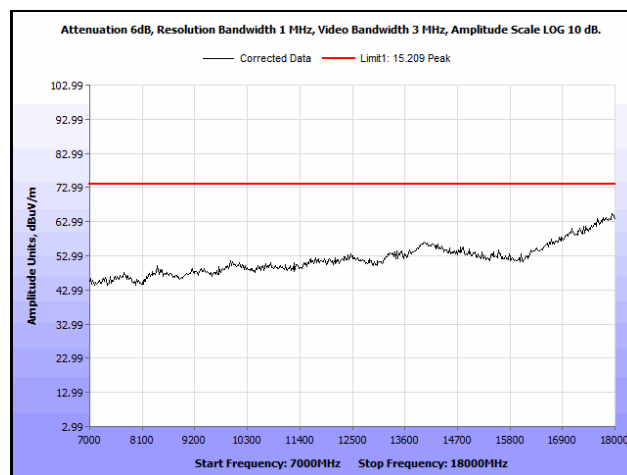
Plot 648. Radiated Spurious Emissions, 802.11ac 20 MHz, Channel 144, 3SS, 7 GHz – 18 GHz, Peak
