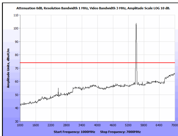
Plot 541. Radiated Spurious Emissions, 802.11a 20 MH, Channel 64, 1 GHz – 7 GHz, Peak
