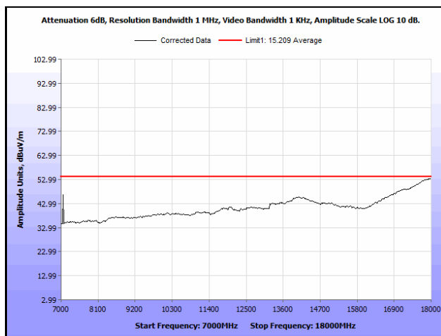
Plot 757. Radiated Spurious Emissions, 802.11ac 80 MH, Channel 58, 3SS, 7 GHz – 18 GHz, Average
