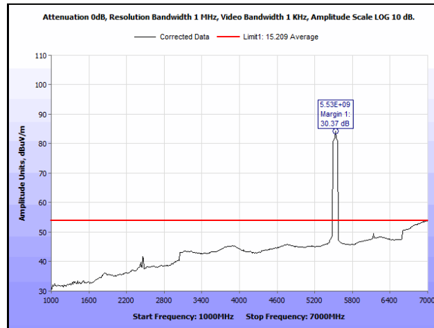
Plot 760. Radiated Spurious Emissions, 802.11ac 80 MHz, Channel 106, 3SS, 1 GHz – 7 GHz, Average
