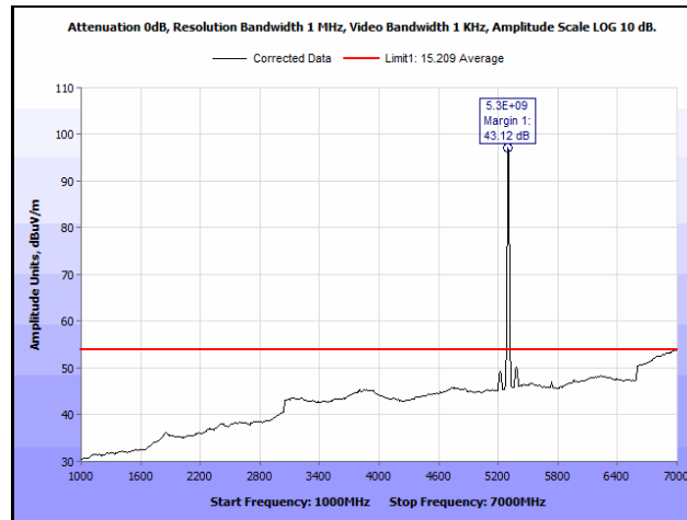
Plot 565. Radiated Spurious Emissions, 802.11ac 20 MHz, Channel 60, 1SS, 1 GHz – 7 GHz, Average
