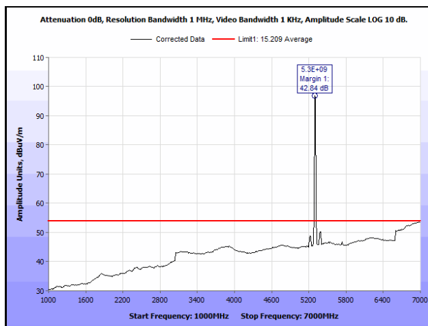
Plot 625. Radiated Spurious Emissions, 802.11ac 20 MHz, Channel 60, 3SS, 1 GHz – 7 GHz, Average
