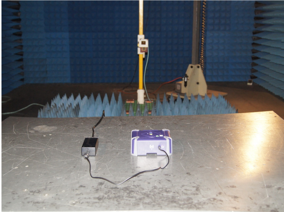
Photograph 4: Set-up for Spurious Emissions (26GHz-40GHz)
