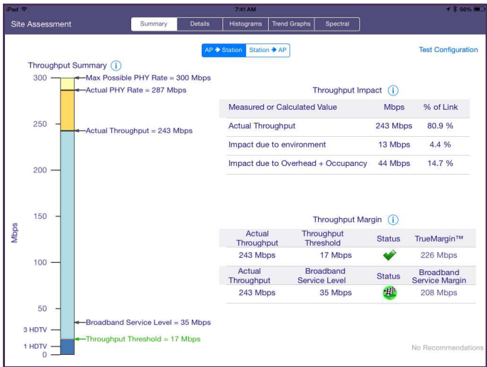
Figure 12 Example of Site Assessment Summary Results
