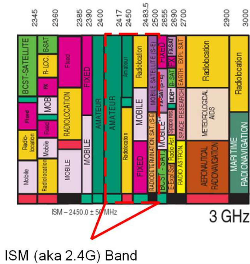
Figure 16 2.4G channel allocation
