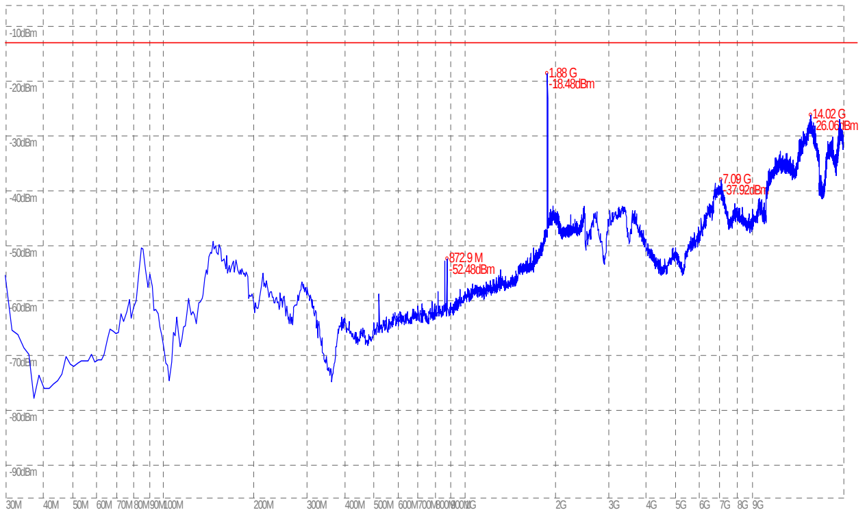
(Plot D.3: EGPRS 1900MHz Channel = 661, Test Antenna Horizontal)
