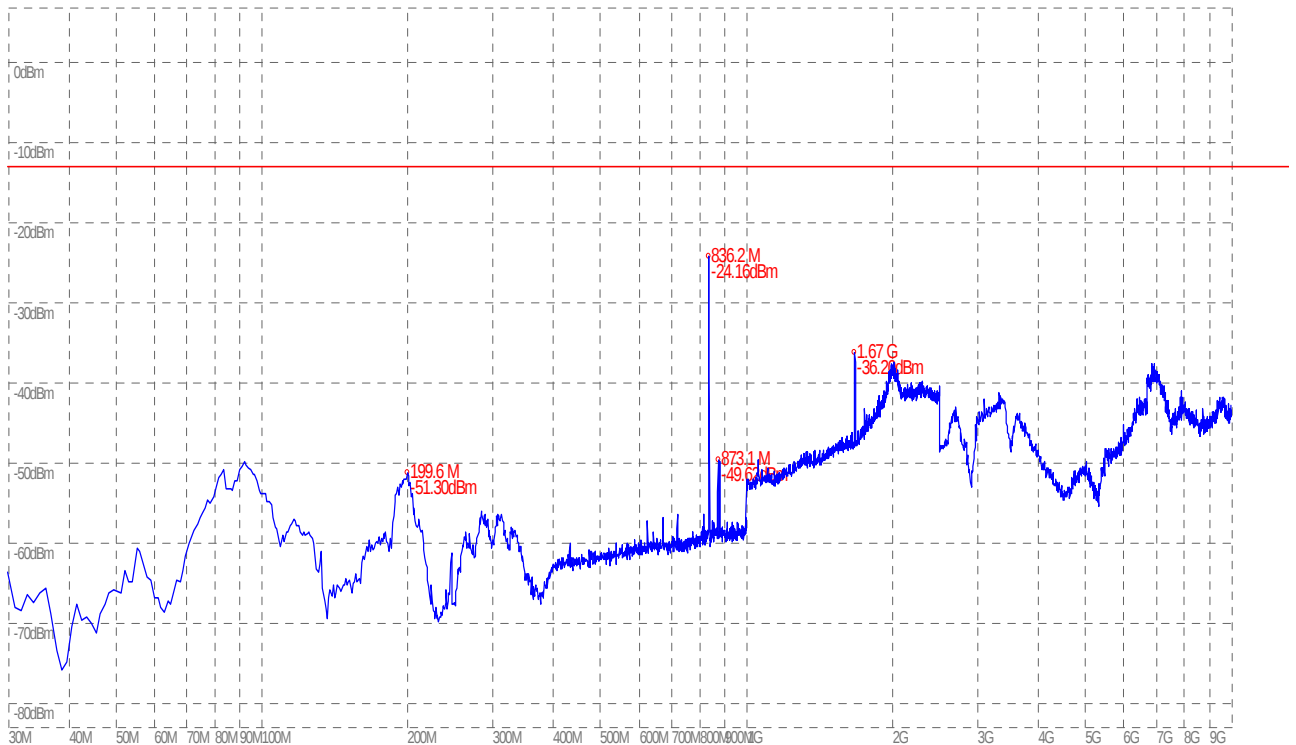
(Plot A.3: GSM 850MHz Channel = 190, Test Antenna Horizontal)
