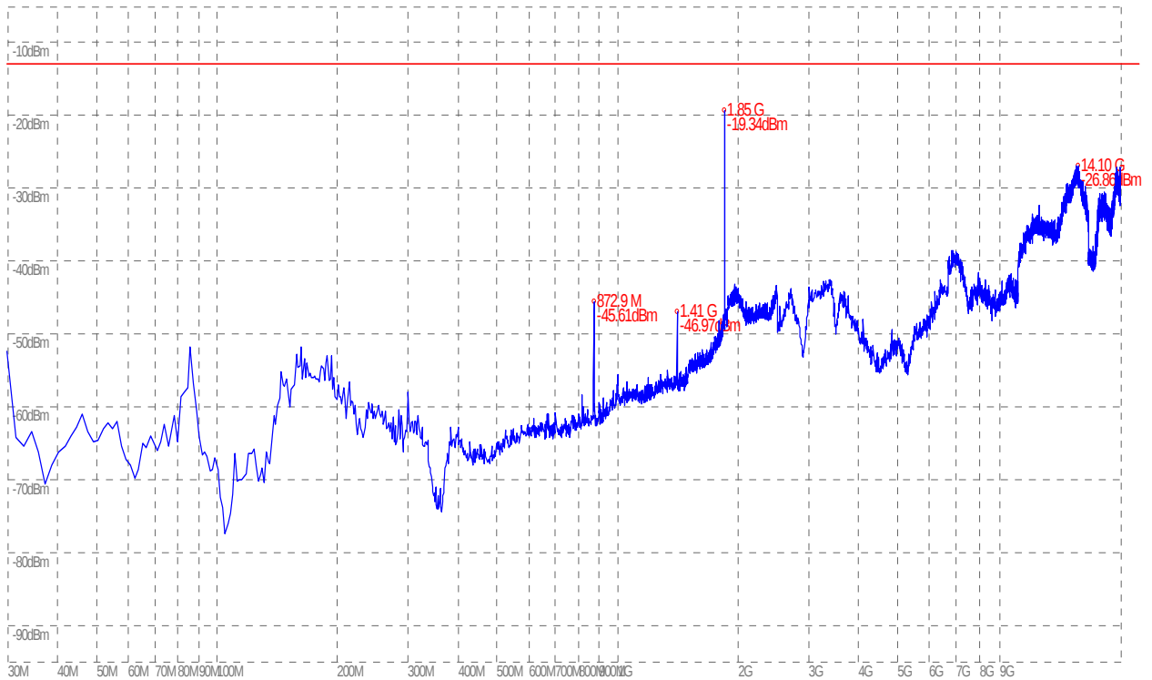
(Plot D.2: EGPRS 1900MHz Channel = 512, Test Antenna Vertical)
