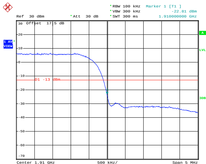
Higher Band Edge Plot on Channel 9538 (1907.6 MHz)
