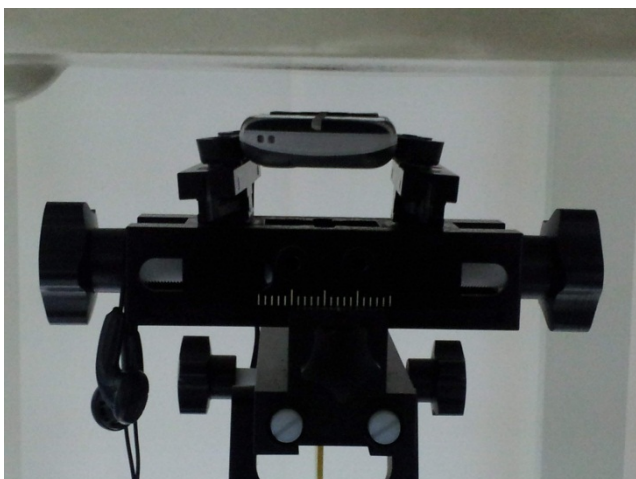
Front of the DUT with Phantom 1.5 cm Gap (w/ headset)
