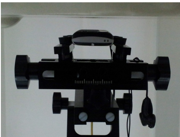
Back of the DUT with Phantom 1.5 cm Gap (w/ headset)
