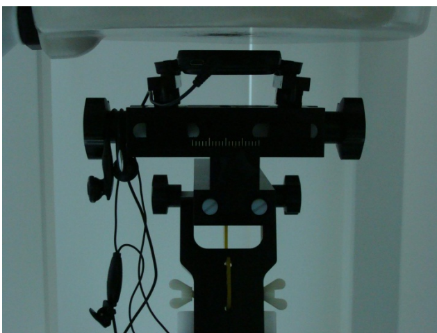
Front of the DUT with Earphone to phantom 1 cm gap
