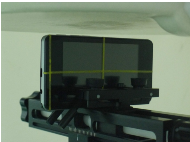
Right Side of the DUT with Phantom 1 cm
