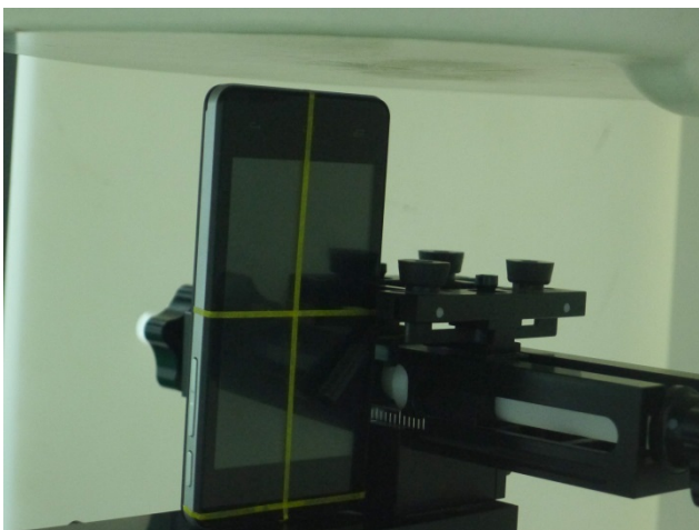
Bottom Side of the DUT with Phantom 1 cm
