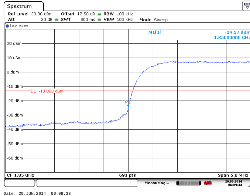
Lower Band Edge Plot on Channel 9262 (1852.4 MHz)
